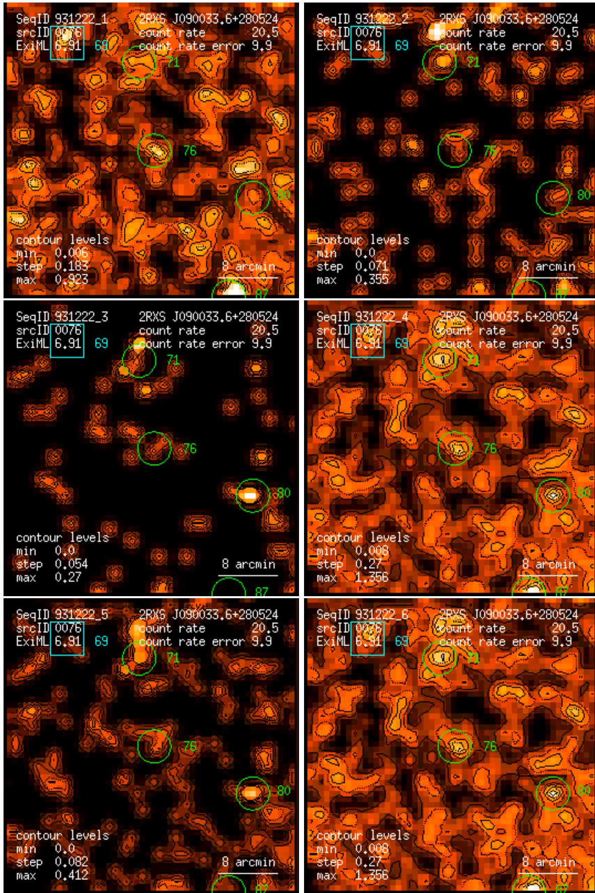
Figure 76: RASS 931222: detection 0076: band rate images, Gaussian filter: (1) PSPC channels 11 – 41, (2) 52 – 90, (3) 91 – 201, (4) 11 – 235, (5) 52 – 201, (6) 11 – 201. Broad band rates in counts/ks. Band rate contour levels in counts/ks/arcmin 2 .
