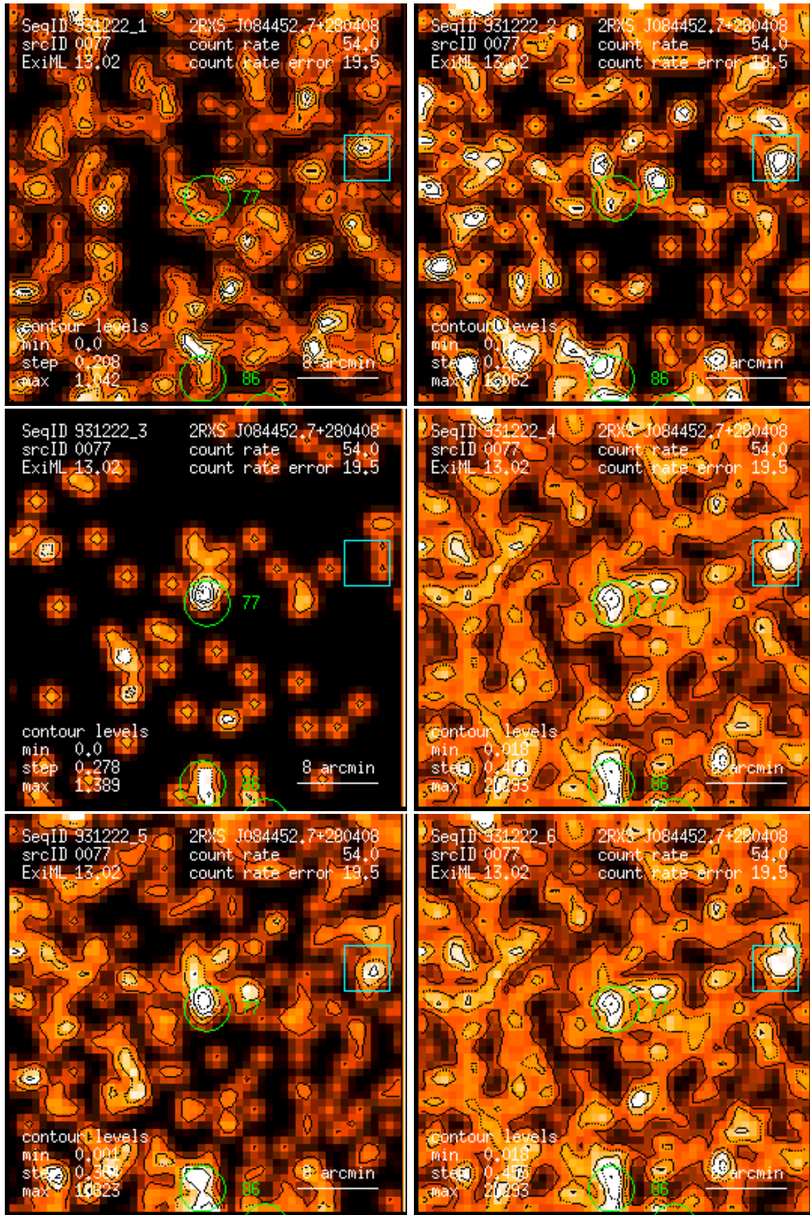
Figure 77: RASS 931222: detection 0077: band rate images, Gaussian filter: (1) PSPC channels 11 – 41, (2) 52 – 90, (3) 91 – 201, (4) 11 – 235, (5) 52 – 201, (6) 11 – 201. Broad band rates in counts/ks. Band rate contour levels in counts/ks/arcmin 2 .
