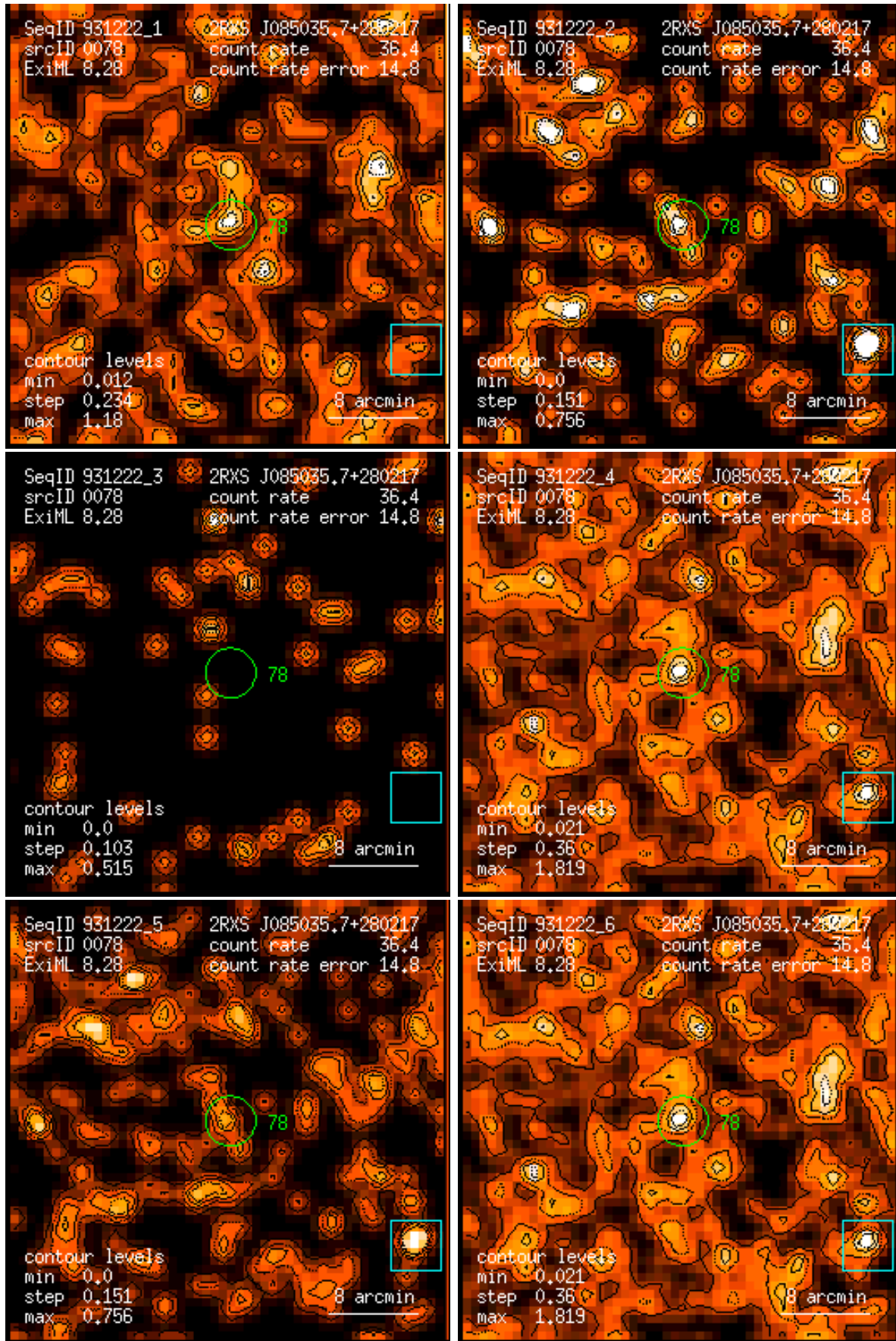
Figure 78: RASS 931222: detection 0078: band rate images, Gaussian filter: (1) PSPC channels 11 – 41, (2) 52 – 90, (3) 91 – 201, (4) 11 – 235, (5) 52 – 201, (6) 11 – 201. Broad band rates in counts/ks. Band rate contour levels in counts/ks/arcmin 2 .
