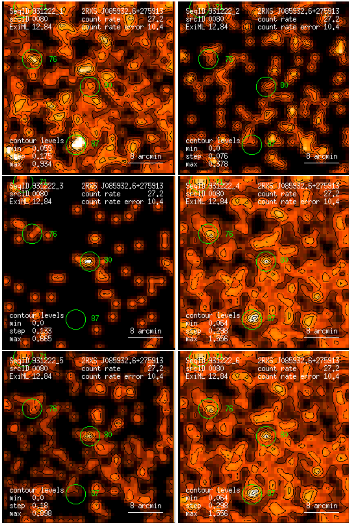
Figure 80: RASS 931222: detection 0080: band rate images, Gaussian filter: (1) PSPC channels 11 – 41, (2) 52 – 90, (3) 91 – 201, (4) 11 – 235, (5) 52 – 201, (6) 11 – 201. Broad band rates in counts/ks. Band rate contour levels in counts/ks/arcmin 2 .
