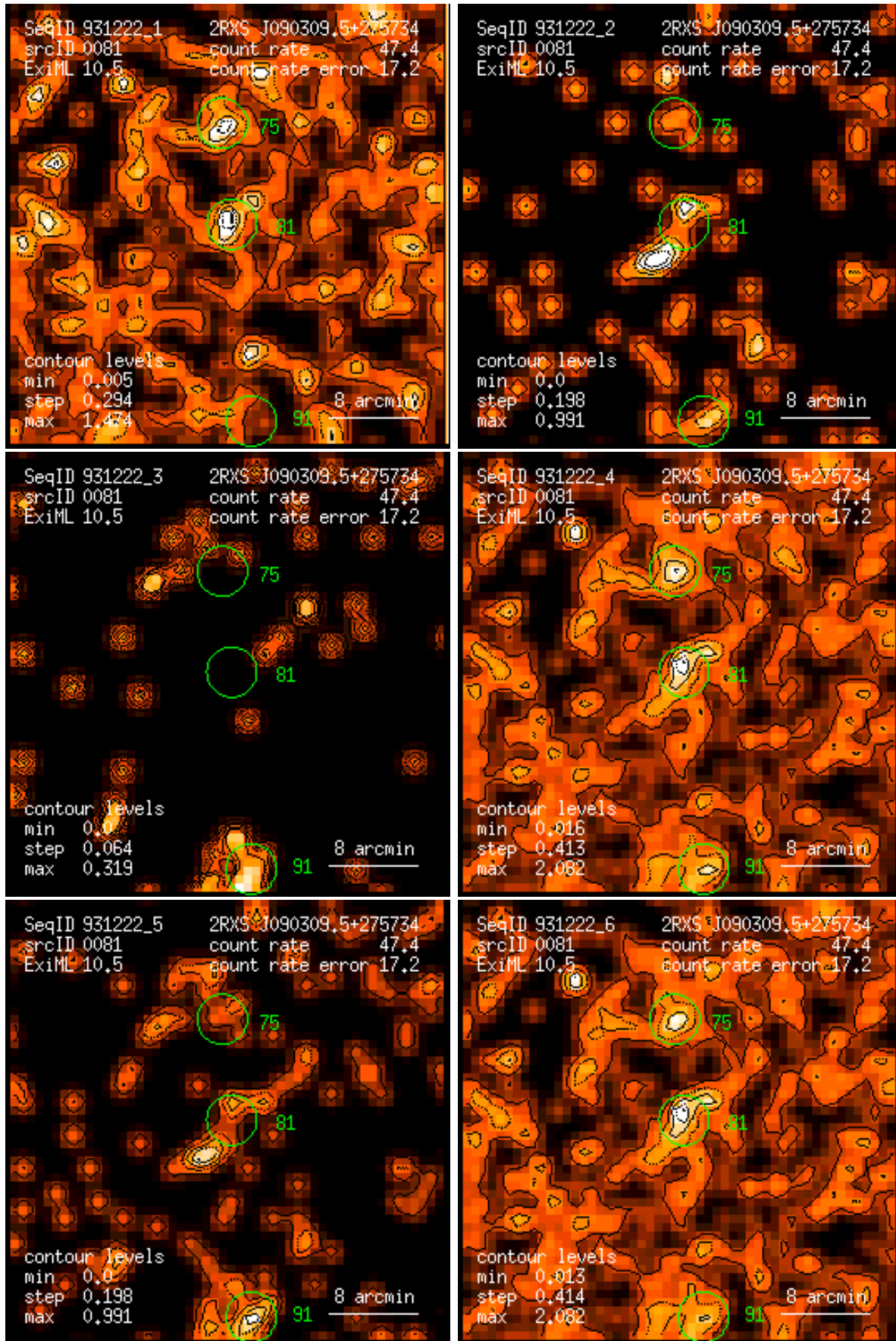
Figure 81: RASS 931222: detection 0081: band rate images, Gaussian filter: (1) PSPC channels 11 – 41, (2) 52 – 90, (3) 91 – 201, (4) 11 – 235, (5) 52 – 201, (6) 11 – 201. Broad band rates in counts/ks. Band rate contour levels in counts/ks/arcmin 2 .
