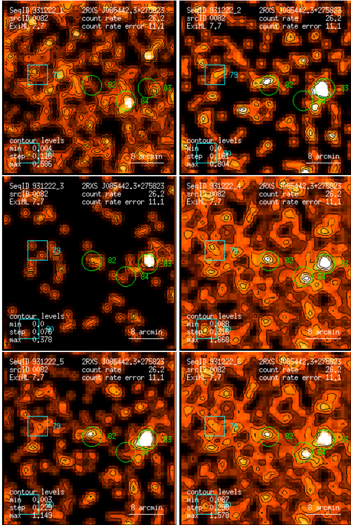
Figure 82: RASS 931222: detection 0082: band rate images, Gaussian filter: (1) PSPC channels 11 – 41, (2) 52 – 90, (3) 91 – 201, (4) 11 – 235, (5) 52 – 201, (6) 11 – 201. Broad band rates in counts/ks. Band rate contour levels in counts/ks/arcmin 2 .
