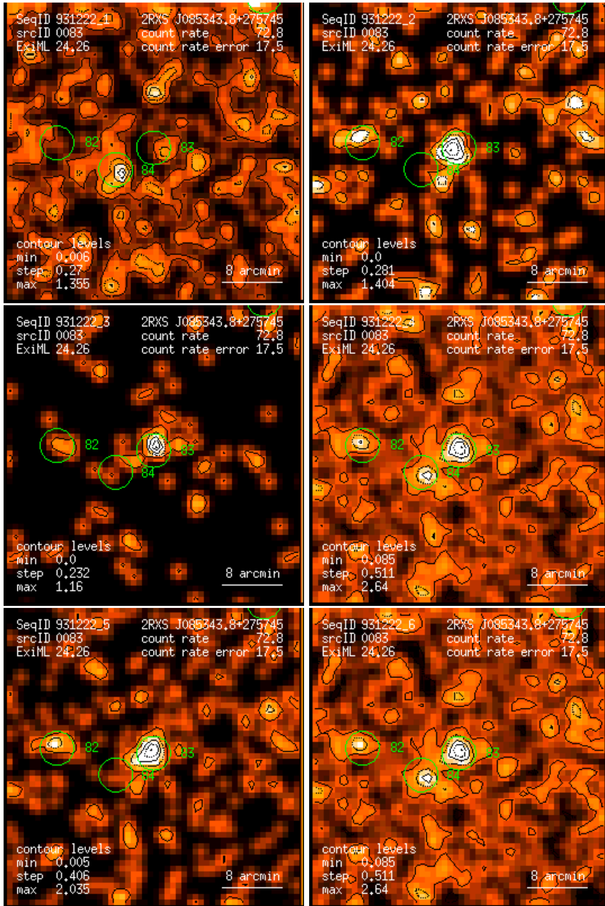
Figure 83: RASS 931222: detection 0083: band rate images, Gaussian filter: (1) PSPC channels 11 – 41, (2) 52 – 90, (3) 91 – 201, (4) 11 – 235, (5) 52 – 201, (6) 11 – 201. Broad band rates in counts/ks. Band rate contour levels in counts/ks/arcmin 2 .
