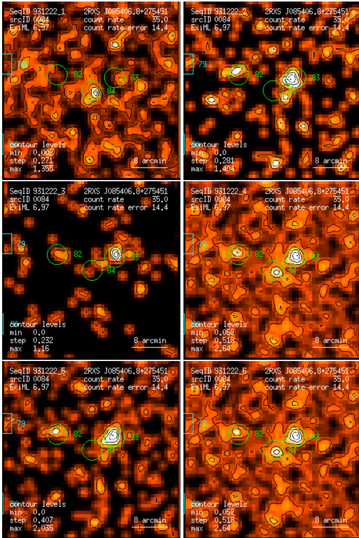
Figure 84: RASS 931222: detection 0084: band rate images, Gaussian filter: (1) PSPC channels 11 – 41, (2) 52 – 90, (3) 91 – 201, (4) 11 – 235, (5) 52 – 201, (6) 11 – 201. Broad band rates in counts/ks. Band rate contour levels in counts/ks/arcmin 2 .
