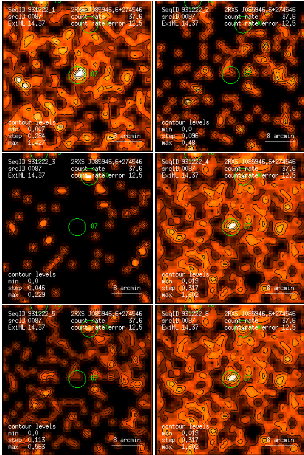
Figure 87: RASS 931222: detection 0087: band rate images, Gaussian filter: (1) PSPC channels 11 – 41, (2) 52 – 90, (3) 91 – 201, (4) 11 – 235, (5) 52 – 201, (6) 11 – 201. Broad band rates in counts/ks. Band rate contour levels in counts/ks/arcmin 2 .
