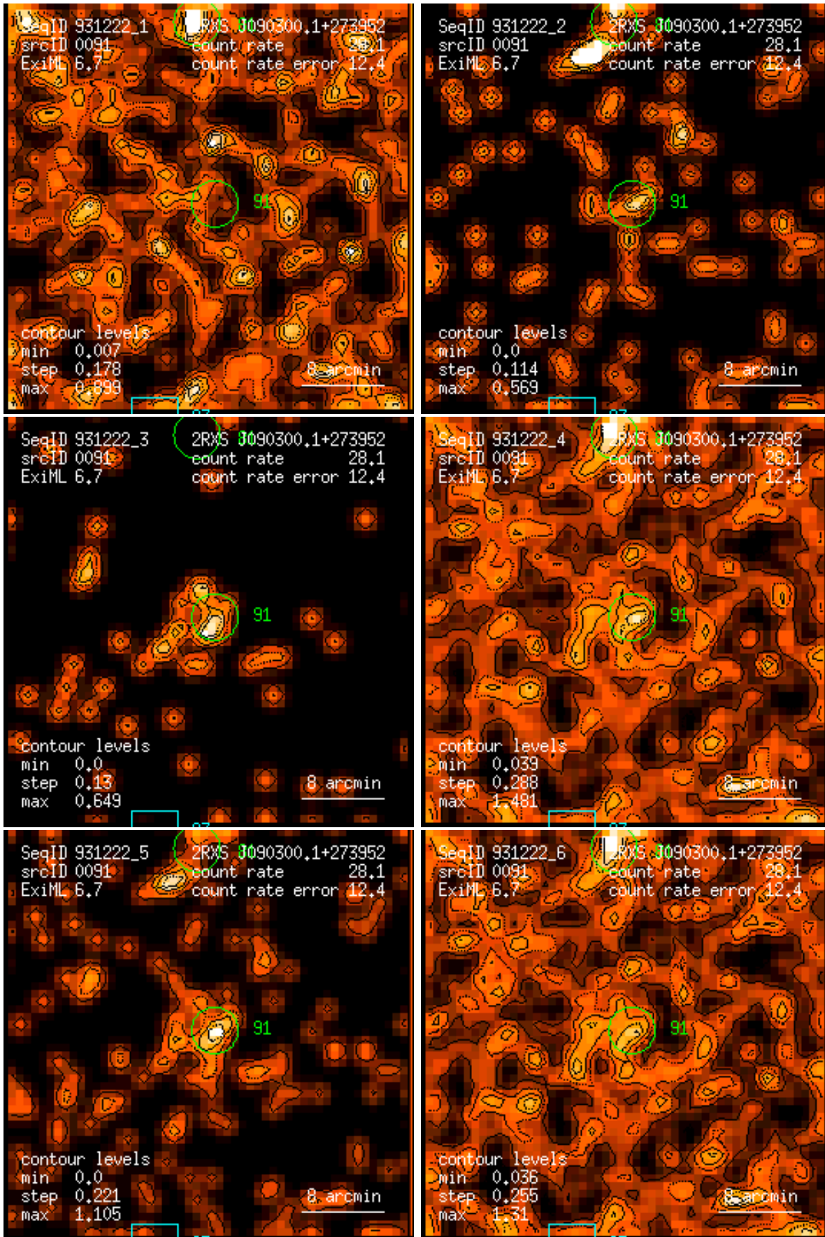
Figure 91: RASS 931222: detection 0091: band rate images, Gaussian filter: (1) PSPC channels 11 – 41, (2) 52 – 90, (3) 91 – 201, (4) 11 – 235, (5) 52 – 201, (6) 11 – 201. Broad band rates in counts/ks. Band rate contour levels in counts/ks/arcmin 2 .
