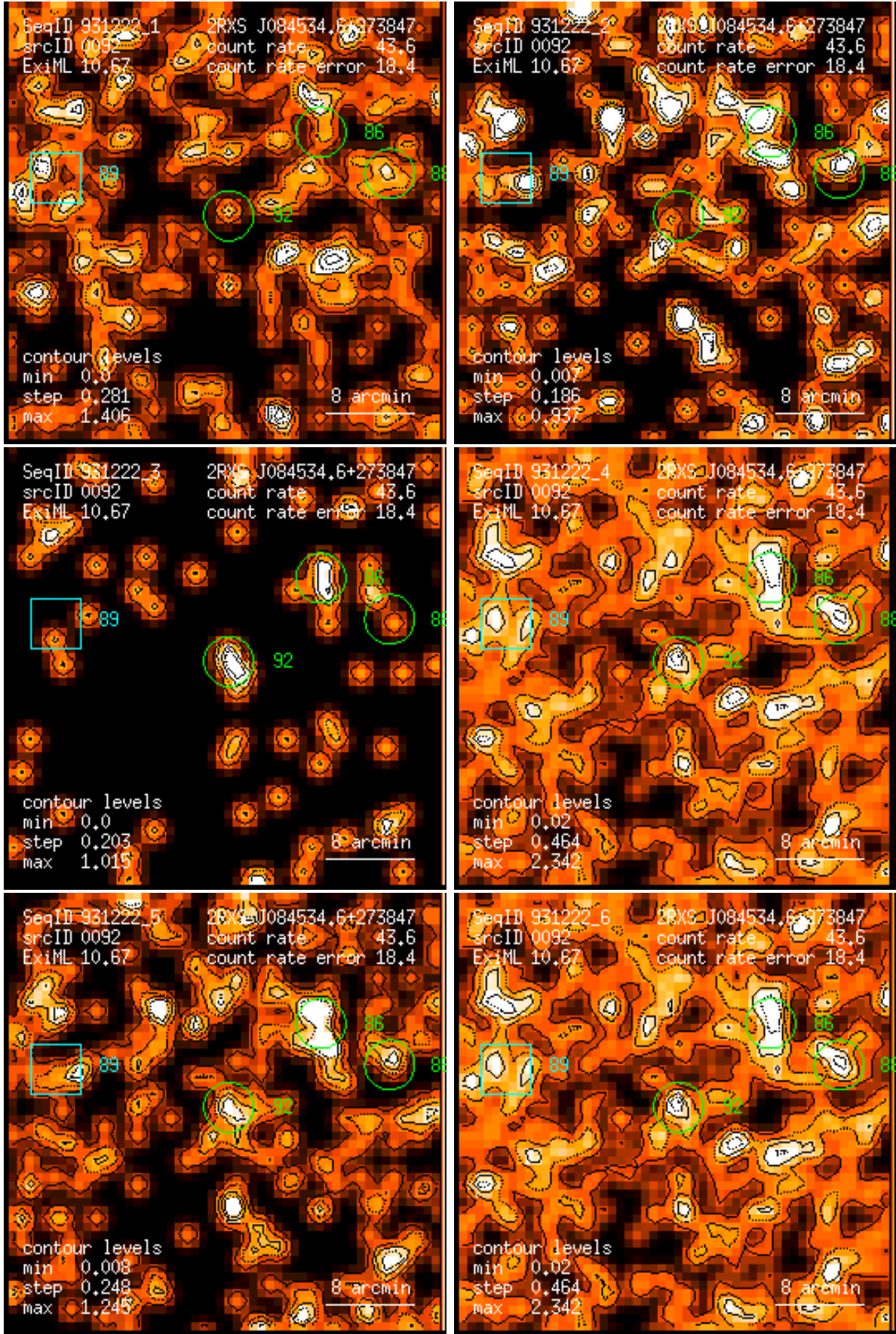
Figure 92: RASS 931222: detection 0092: band rate images, Gaussian filter: (1) PSPC channels 11 – 41, (2) 52 – 90, (3) 91 – 201, (4) 11 – 235, (5) 52 – 201, (6) 11 – 201. Broad band rates in counts/ks. Band rate contour levels in counts/ks/arcmin 2 .
