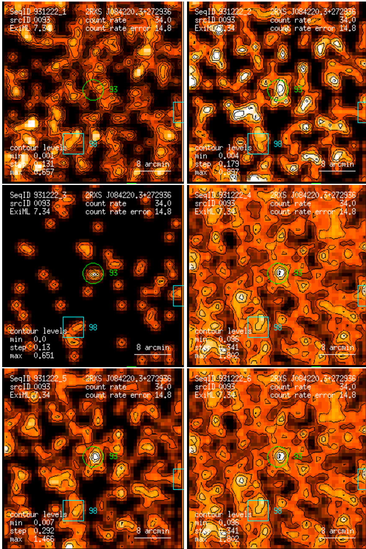
Figure 93: RASS 931222: detection 0093: band rate images, Gaussian filter: (1) PSPC channels 11 – 41, (2) 52 – 90, (3) 91 – 201, (4) 11 – 235, (5) 52 – 201, (6) 11 – 201. Broad band rates in counts/ks. Band rate contour levels in counts/ks/arcmin 2 .
