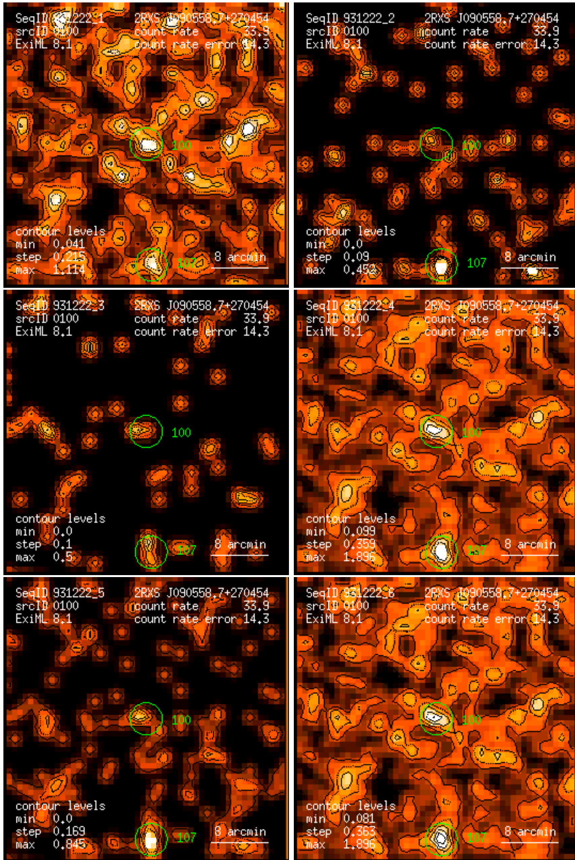
Figure 100: RASS 931222: detection 0100: band rate images, Gaussian filter: (1) PSPC channels 11 – 41, (2) 52 – 90, (3) 91 – 201, (4) 11 – 235, (5) 52 – 201, (6) 11 – 201. Broad band rates in counts/ks. Band rate contour levels in counts/ks/arcmin 2 .
