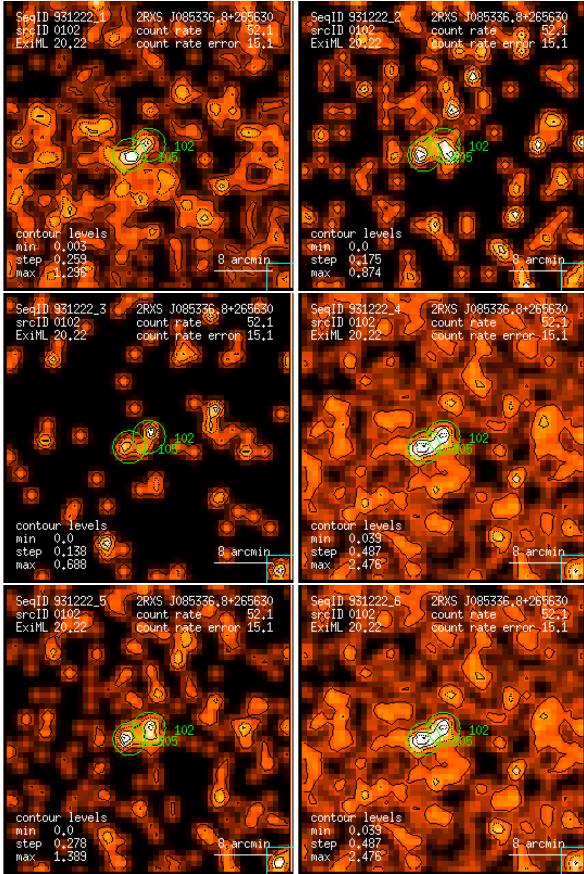
Figure 102: RASS 931222: detection 0102: band rate images, Gaussian filter: (1) PSPC channels 11 – 41, (2) 52 – 90, (3) 91 – 201, (4) 11 – 235, (5) 52 – 201, (6) 11 – 201. Broad band rates in counts/ks. Band rate contour levels in counts/ks/arcmin 2 .
