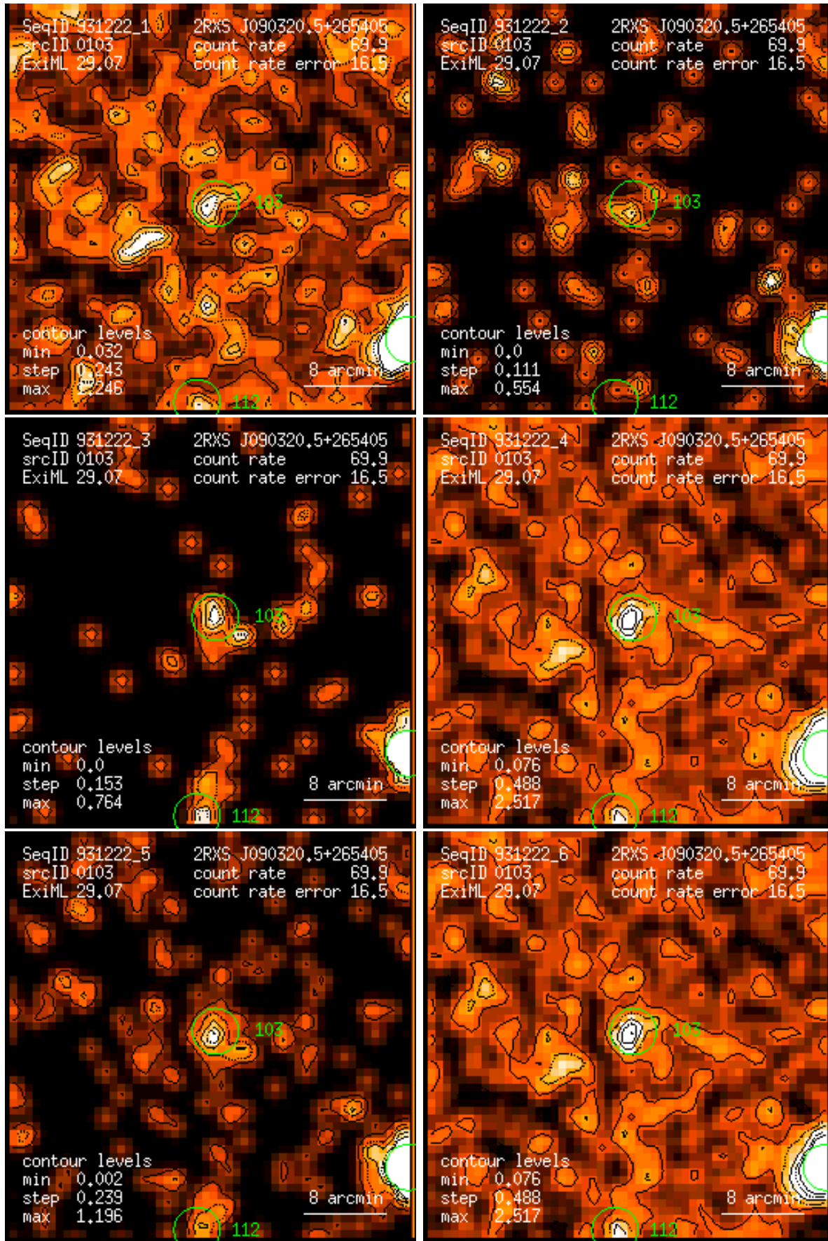
Figure 103: RASS 931222: detection 0103: band rate images, Gaussian filter: (1) PSPC channels 11 – 41, (2) 52 – 90, (3) 91 – 201, (4) 11 – 235, (5) 52 – 201, (6) 11 – 201. Broad band rates in counts/ks. Band rate contour levels in counts/ks/arcmin 2 .
