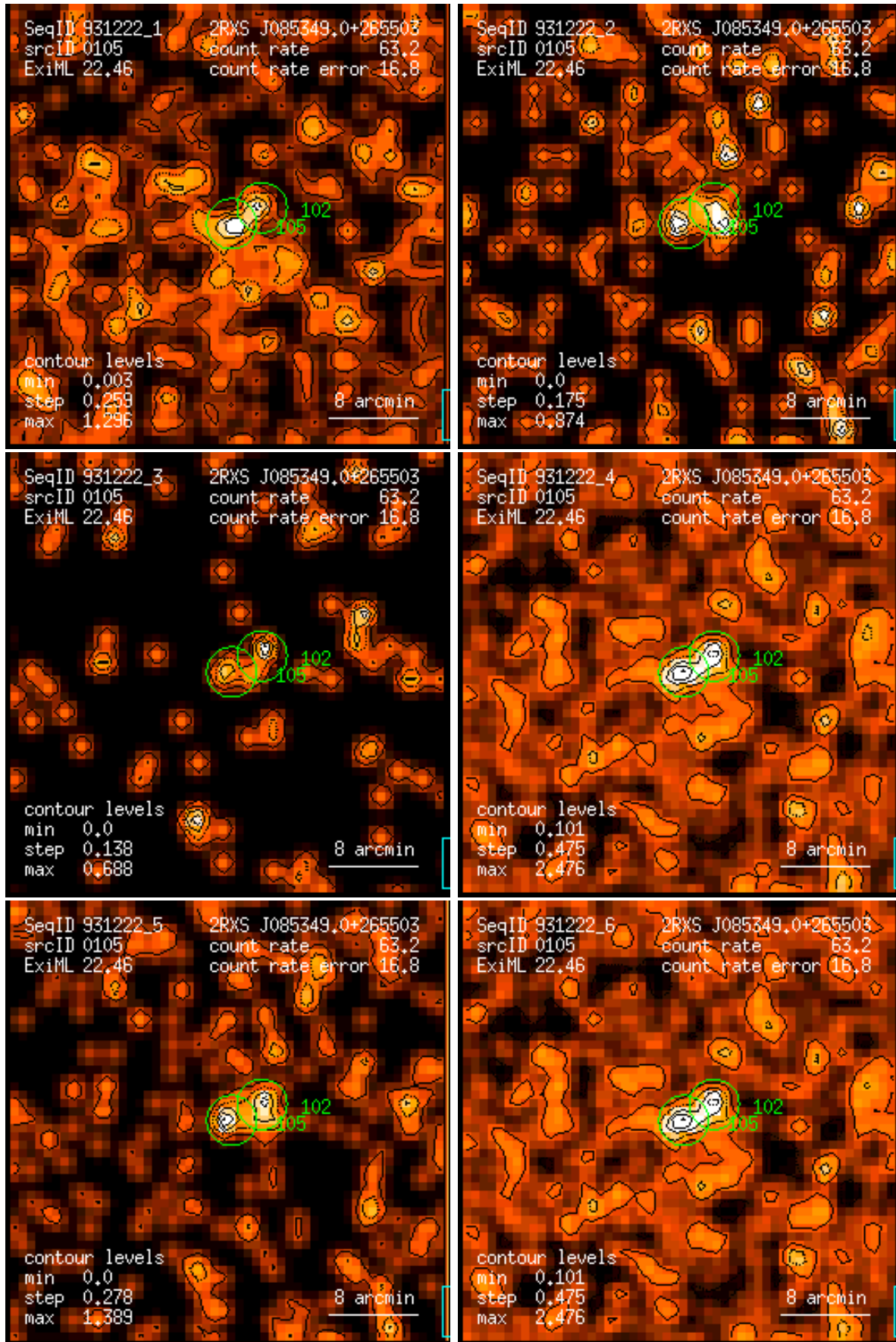
Figure 105: RASS 931222: detection 0105: band rate images, Gaussian filter: (1) PSPC channels 11 – 41, (2) 52 – 90, (3) 91 – 201, (4) 11 – 235, (5) 52 – 201, (6) 11 – 201. Broad band rates in counts/ks. Band rate contour levels in counts/ks/arcmin 2 .
