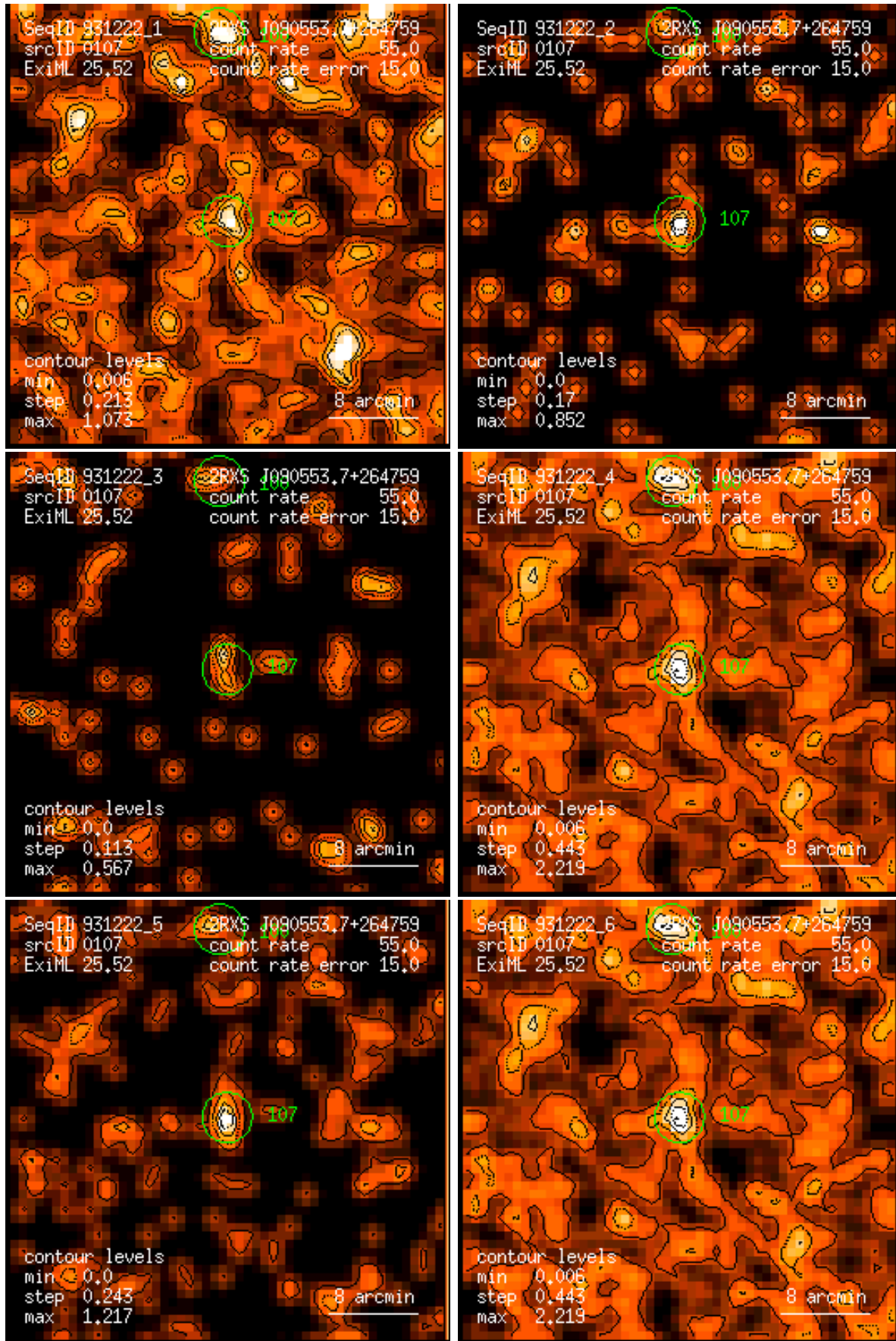
Figure 107: RASS 931222: detection 0107: band rate images, Gaussian filter: (1) PSPC channels 11 – 41, (2) 52 – 90, (3) 91 – 201, (4) 11 – 235, (5) 52 – 201, (6) 11 – 201. Broad band rates in counts/ks. Band rate contour levels in counts/ks/arcmin 2 .
