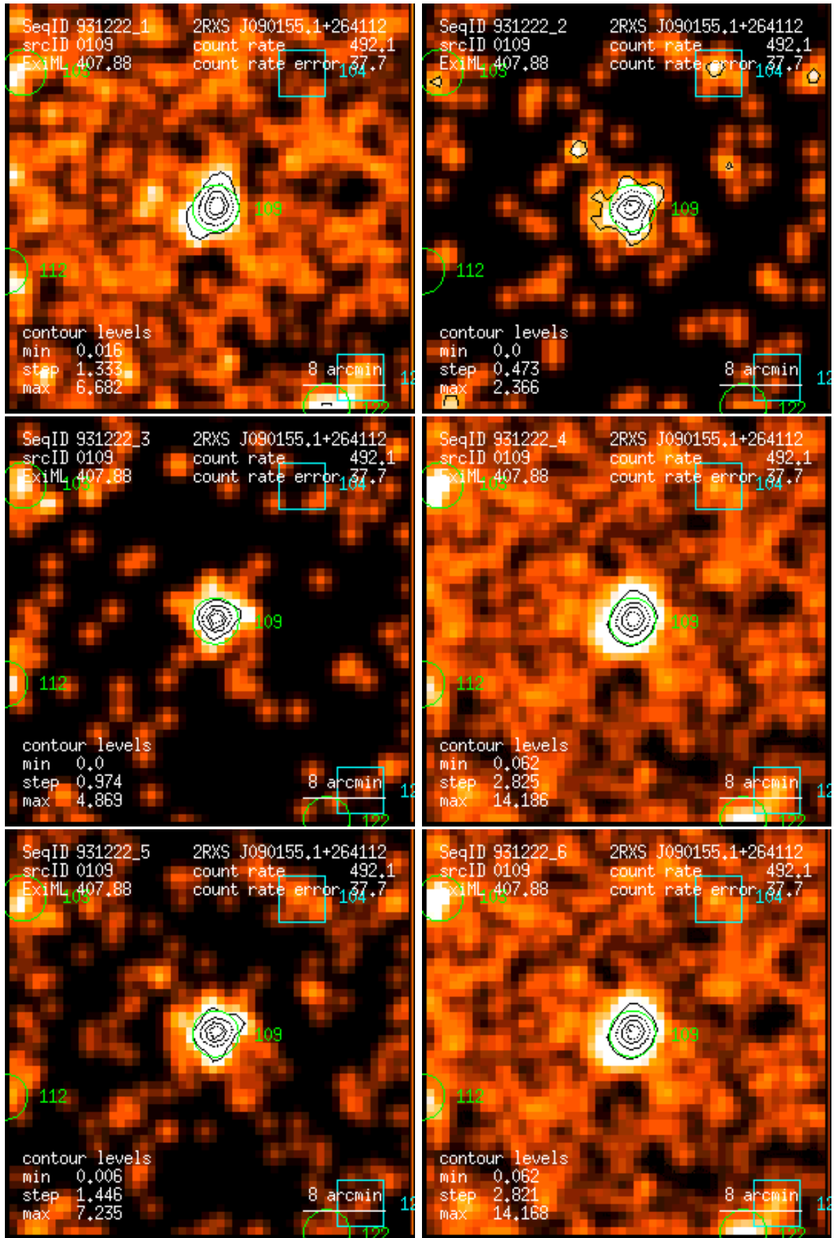
Figure 109: RASS 931222: detection 0109: band rate images, Gaussian filter: (1) PSPC channels 11 – 41, (2) 52 – 90, (3) 91 – 201, (4) 11 – 235, (5) 52 – 201, (6) 11 – 201. Broad band rates in counts/ks. Band rate contour levels in counts/ks/arcmin 2 .
