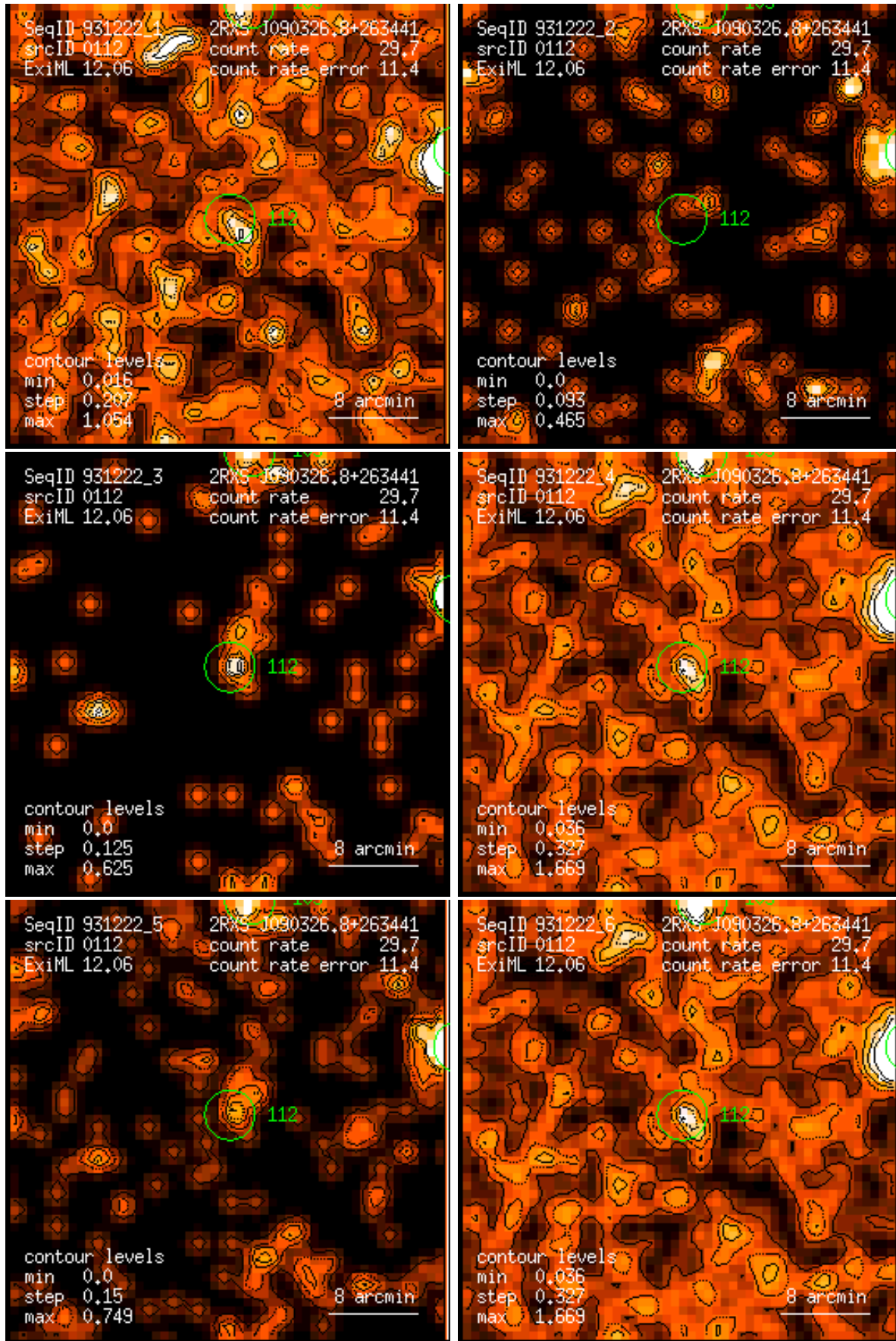
Figure 112: RASS 931222: detection 0112: band rate images, Gaussian filter: (1) PSPC channels 11 – 41, (2) 52 – 90, (3) 91 – 201, (4) 11 – 235, (5) 52 – 201, (6) 11 – 201. Broad band rates in counts/ks. Band rate contour levels in counts/ks/arcmin 2 .
