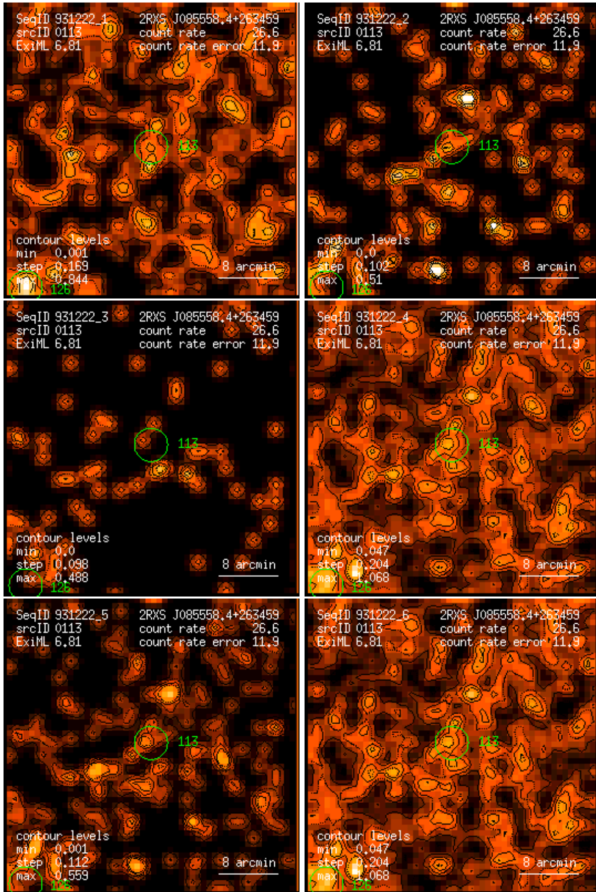
Figure 113: RASS 931222: detection 0113: band rate images, Gaussian filter: (1) PSPC channels 11 – 41, (2) 52 – 90, (3) 91 – 201, (4) 11 – 235, (5) 52 – 201, (6) 11 – 201. Broad band rates in counts/ks. Band rate contour levels in counts/ks/arcmin 2 .
