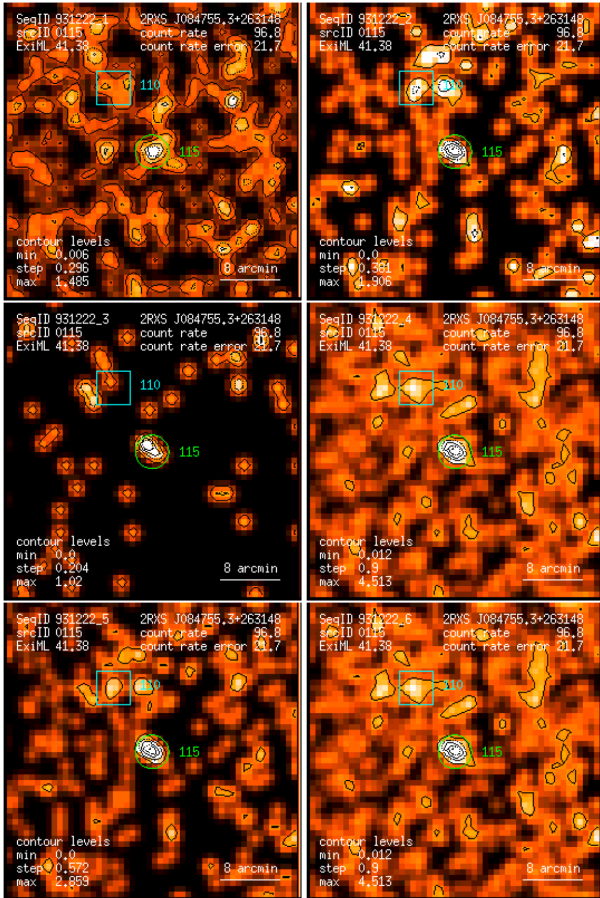
Figure 115: RASS 931222: detection 0115: band rate images, Gaussian filter: (1) PSPC channels 11 – 41, (2) 52 – 90, (3) 91 – 201, (4) 11 – 235, (5) 52 – 201, (6) 11 – 201. Broad band rates in counts/ks. Band rate contour levels in counts/ks/arcmin 2 .
