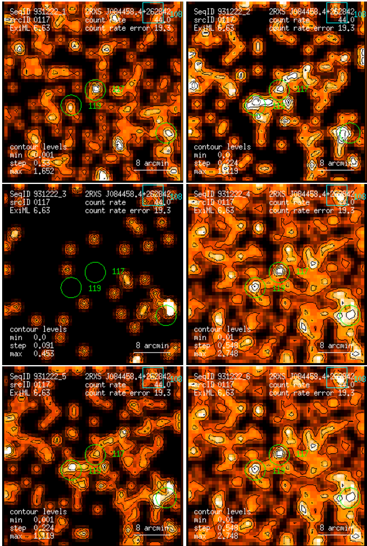
Figure 117: RASS 931222: detection 0117: band rate images, Gaussian filter: (1) PSPC channels 11 – 41, (2) 52 – 90, (3) 91 – 201, (4) 11 – 235, (5) 52 – 201, (6) 11 – 201. Broad band rates in counts/ks. Band rate contour levels in counts/ks/arcmin 2 .
