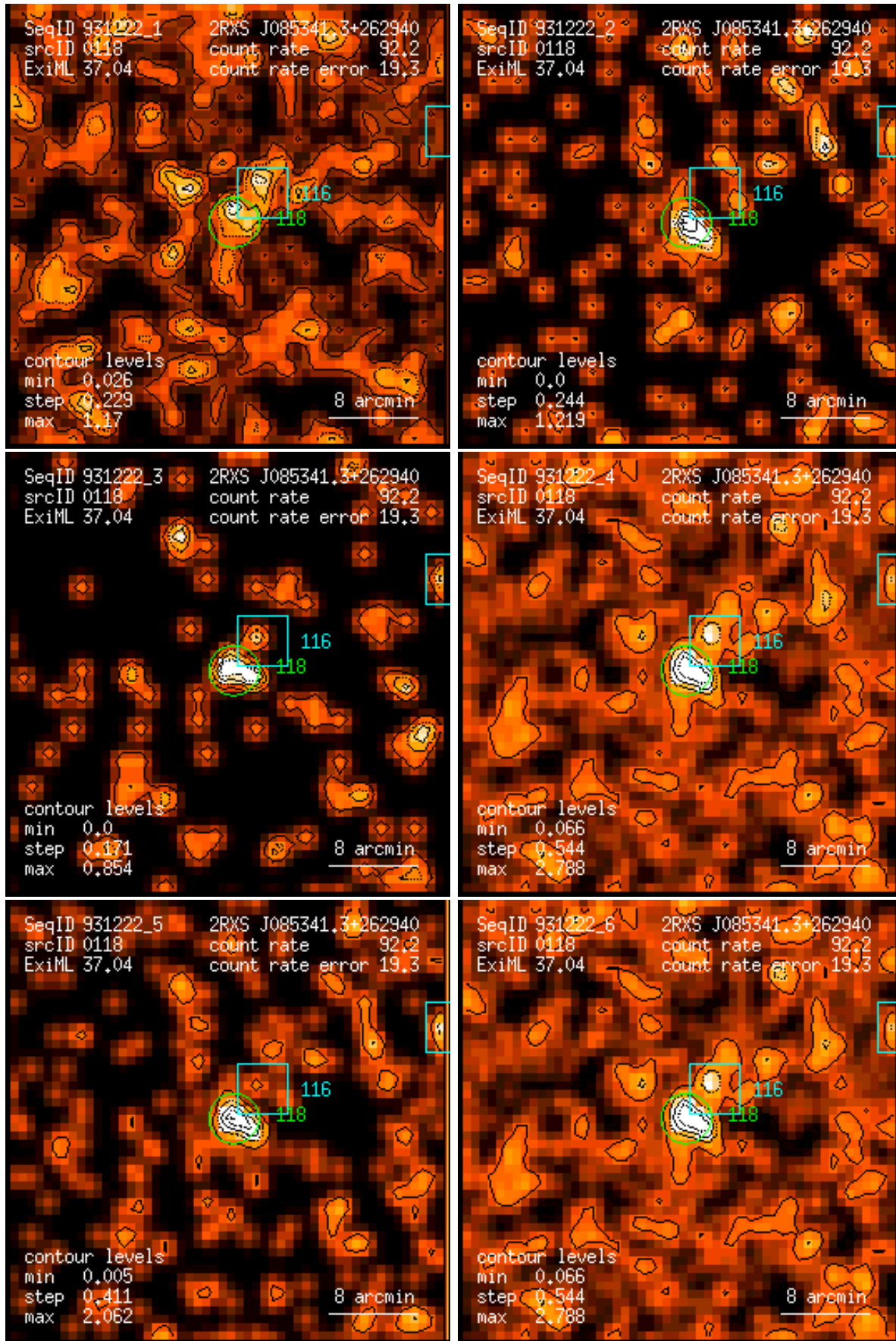
Figure 118: RASS 931222: detection 0118: band rate images, Gaussian filter: (1) PSPC channels 11 – 41, (2) 52 – 90, (3) 91 – 201, (4) 11 – 235, (5) 52 – 201, (6) 11 – 201. Broad band rates in counts/ks. Band rate contour levels in counts/ks/arcmin 2 .
