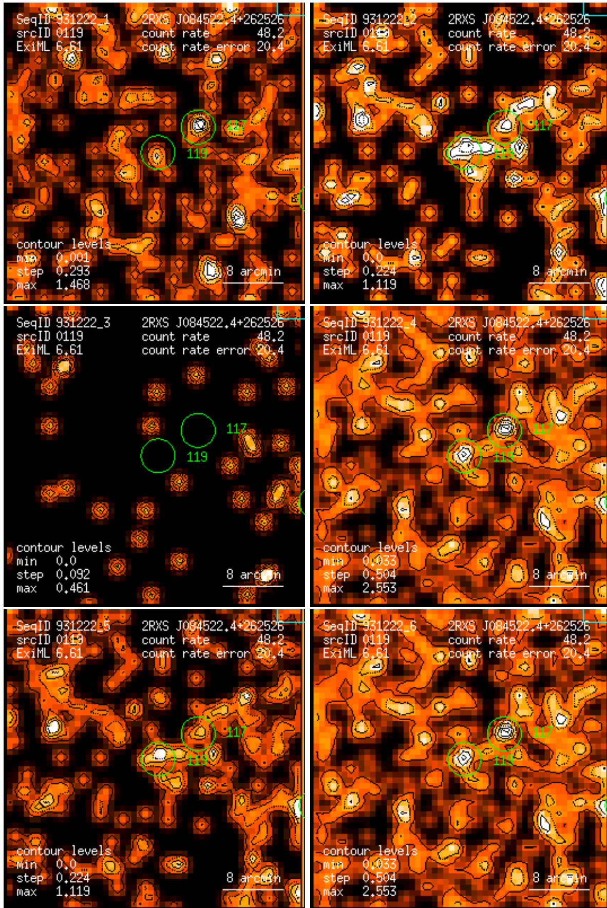
Figure 119: RASS 931222: detection 0119: band rate images, Gaussian filter: (1) PSPC channels 11 – 41, (2) 52 – 90, (3) 91 – 201, (4) 11 – 235, (5) 52 – 201, (6) 11 – 201. Broad band rates in counts/ks. Band rate contour levels in counts/ks/arcmin 2 .
