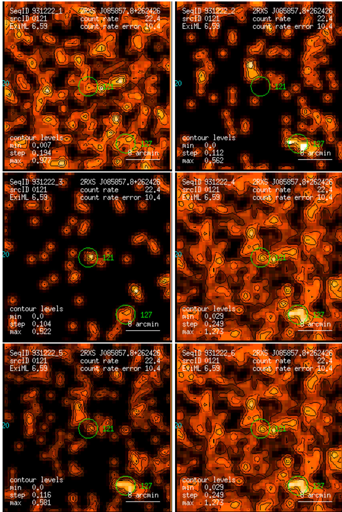
Figure 121: RASS 931222: detection 0121: band rate images, Gaussian filter: (1) PSPC channels 11 – 41, (2) 52 – 90, (3) 91 – 201, (4) 11 – 235, (5) 52 – 201, (6) 11 – 201. Broad band rates in counts/ks. Band rate contour levels in counts/ks/arcmin 2 .
