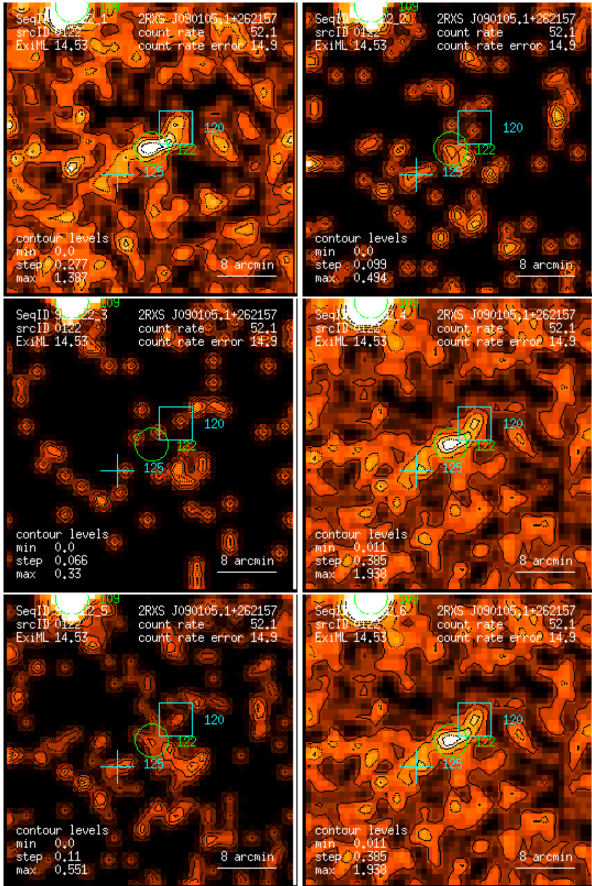
Figure 122: RASS 931222: detection 0122: band rate images, Gaussian filter: (1) PSPC channels 11 – 41, (2) 52 – 90, (3) 91 – 201, (4) 11 – 235, (5) 52 – 201, (6) 11 – 201. Broad band rates in counts/ks. Band rate contour levels in counts/ks/arcmin 2 .
