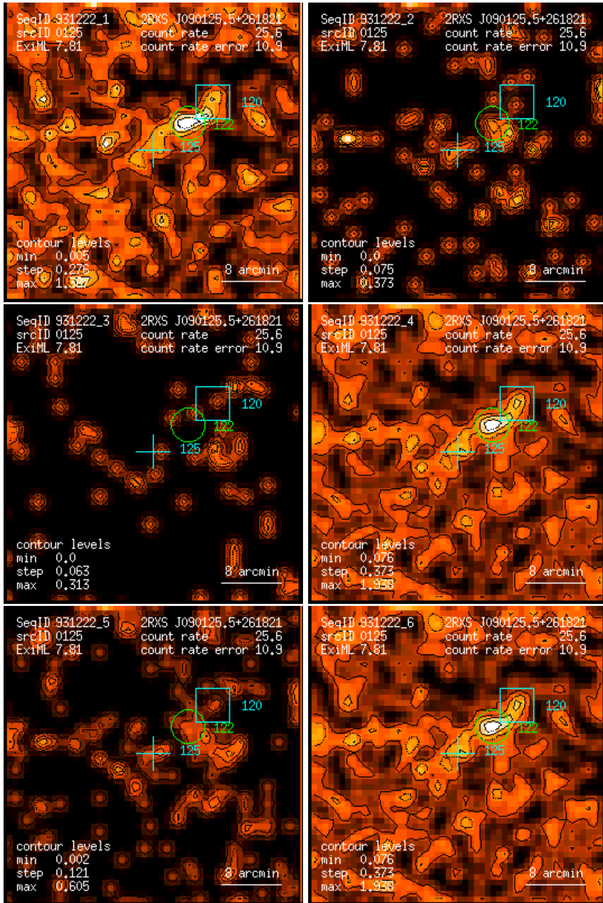
Figure 125: RASS 931222: detection 0125: band rate images, Gaussian filter: (1) PSPC channels 11 – 41, (2) 52 – 90, (3) 91 – 201, (4) 11 – 235, (5) 52 – 201, (6) 11 – 201. Broad band rates in counts/ks. Band rate contour levels in counts/ks/arcmin 2 .
