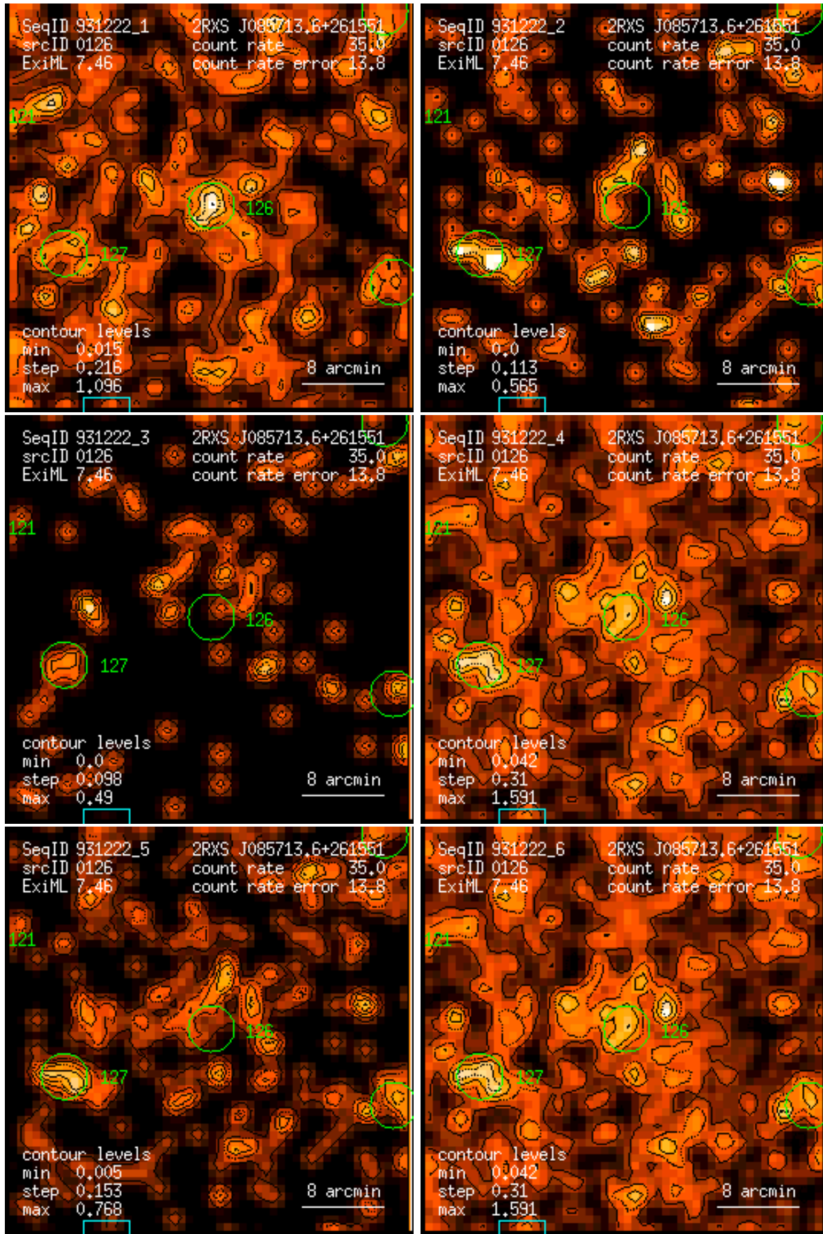
Figure 126: RASS 931222: detection 0126: band rate images, Gaussian filter: (1) PSPC channels 11 – 41, (2) 52 – 90, (3) 91 – 201, (4) 11 – 235, (5) 52 – 201, (6) 11 – 201. Broad band rates in counts/ks. Band rate contour levels in counts/ks/arcmin 2 .
