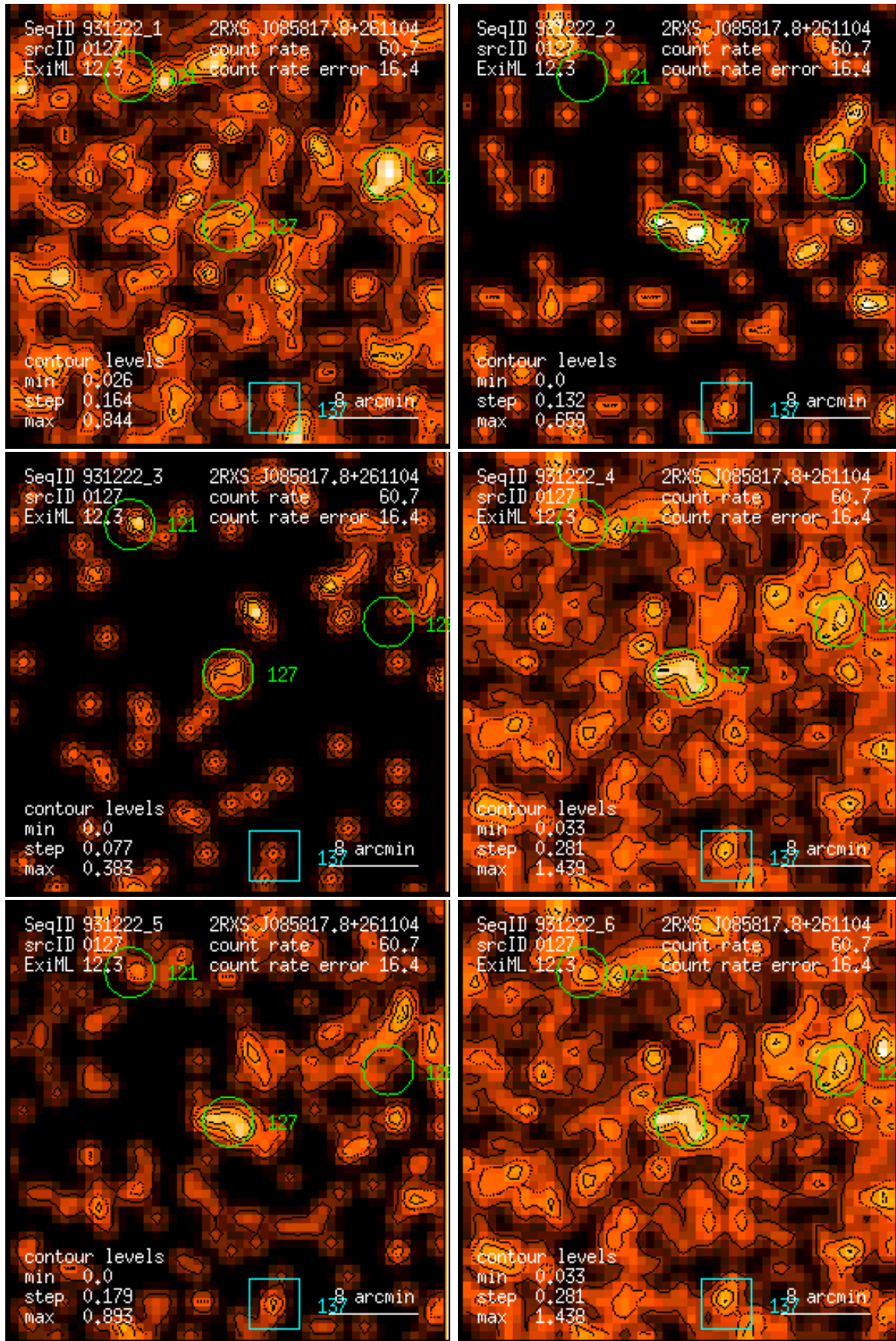
Figure 127: RASS 931222: detection 0127: band rate images, Gaussian filter: (1) PSPC channels 11 – 41, (2) 52 – 90, (3) 91 – 201, (4) 11 – 235, (5) 52 – 201, (6) 11 – 201. Broad band rates in counts/ks. Band rate contour levels in counts/ks/arcmin 2 .
