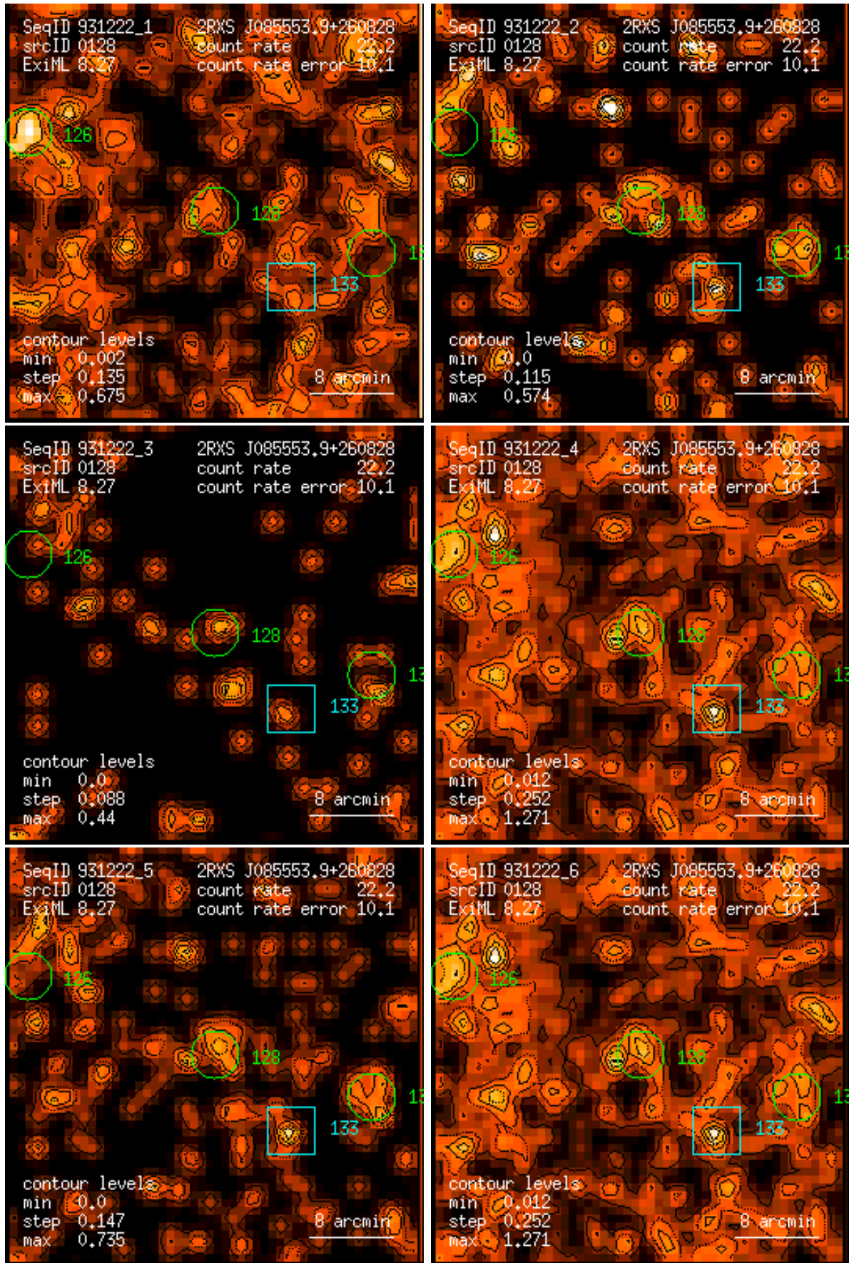
Figure 128: RASS 931222: detection 0128: band rate images, Gaussian filter: (1) PSPC channels 11 – 41, (2) 52 – 90, (3) 91 – 201, (4) 11 – 235, (5) 52 – 201, (6) 11 – 201. Broad band rates in counts/ks. Band rate contour levels in counts/ks/arcmin 2 .
