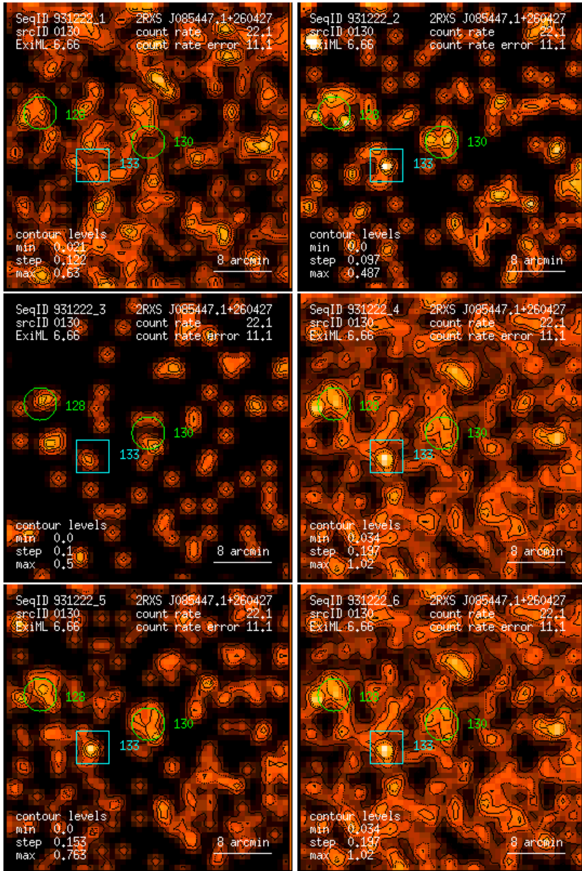
Figure 130: RASS 931222: detection 0130: band rate images, Gaussian filter: (1) PSPC channels 11 – 41, (2) 52 – 90, (3) 91 – 201, (4) 11 – 235, (5) 52 – 201, (6) 11 – 201. Broad band rates in counts/ks. Band rate contour levels in counts/ks/arcmin 2 .
