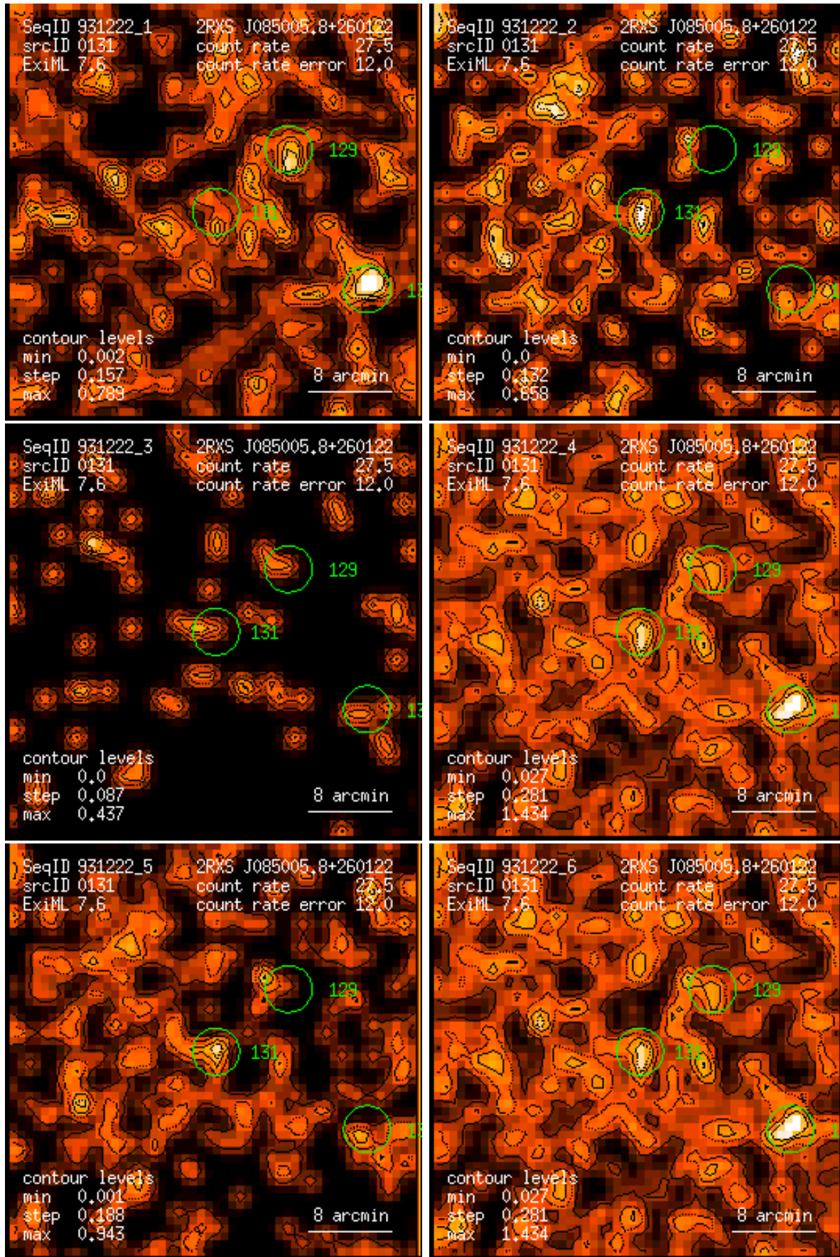
Figure 131: RASS 931222: detection 0131: band rate images, Gaussian filter: (1) PSPC channels 11 – 41, (2) 52 – 90, (3) 91 – 201, (4) 11 – 235, (5) 52 – 201, (6) 11 – 201. Broad band rates in counts/ks. Band rate contour levels in counts/ks/arcmin 2 .
