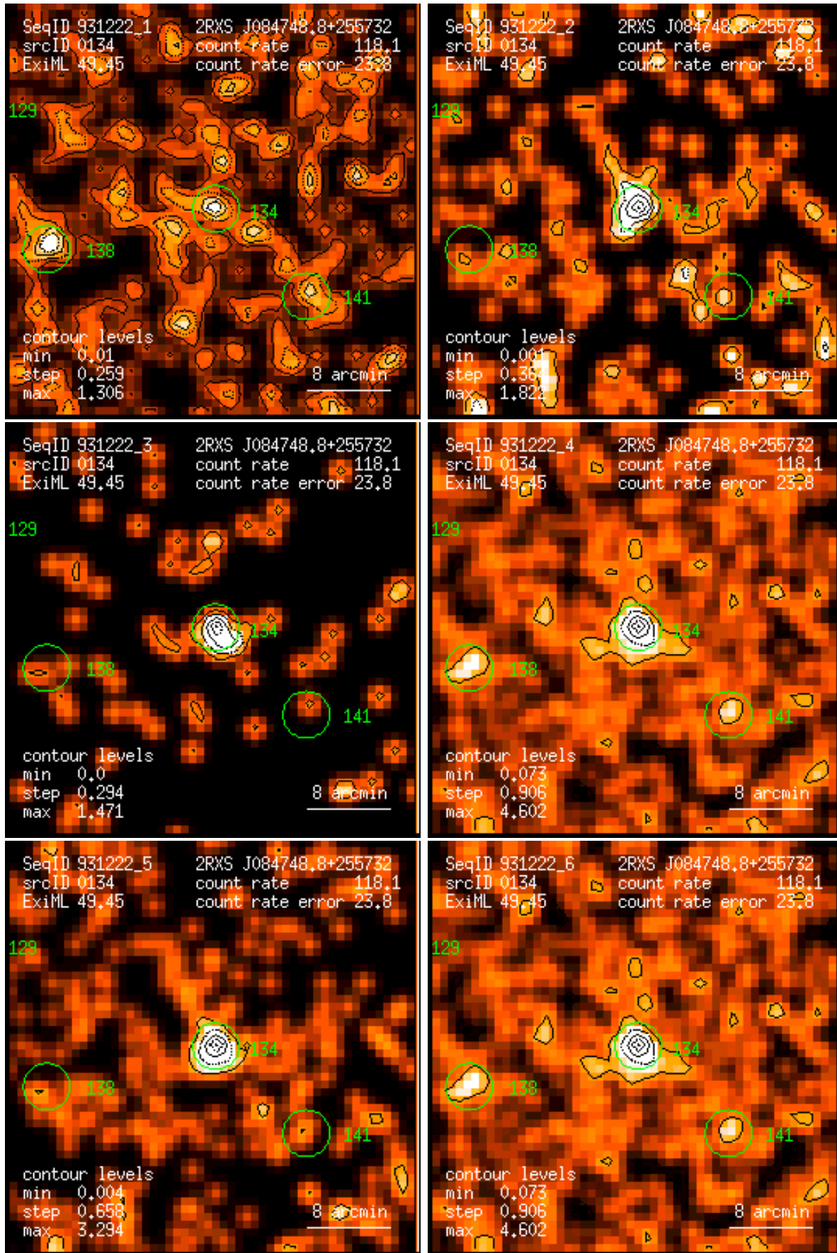
Figure 134: RASS 931222: detection 0134: band rate images, Gaussian filter: (1) PSPC channels 11 – 41, (2) 52 – 90, (3) 91 – 201, (4) 11 – 235, (5) 52 – 201, (6) 11 – 201. Broad band rates in counts/ks. Band rate contour levels in counts/ks/arcmin 2 .
