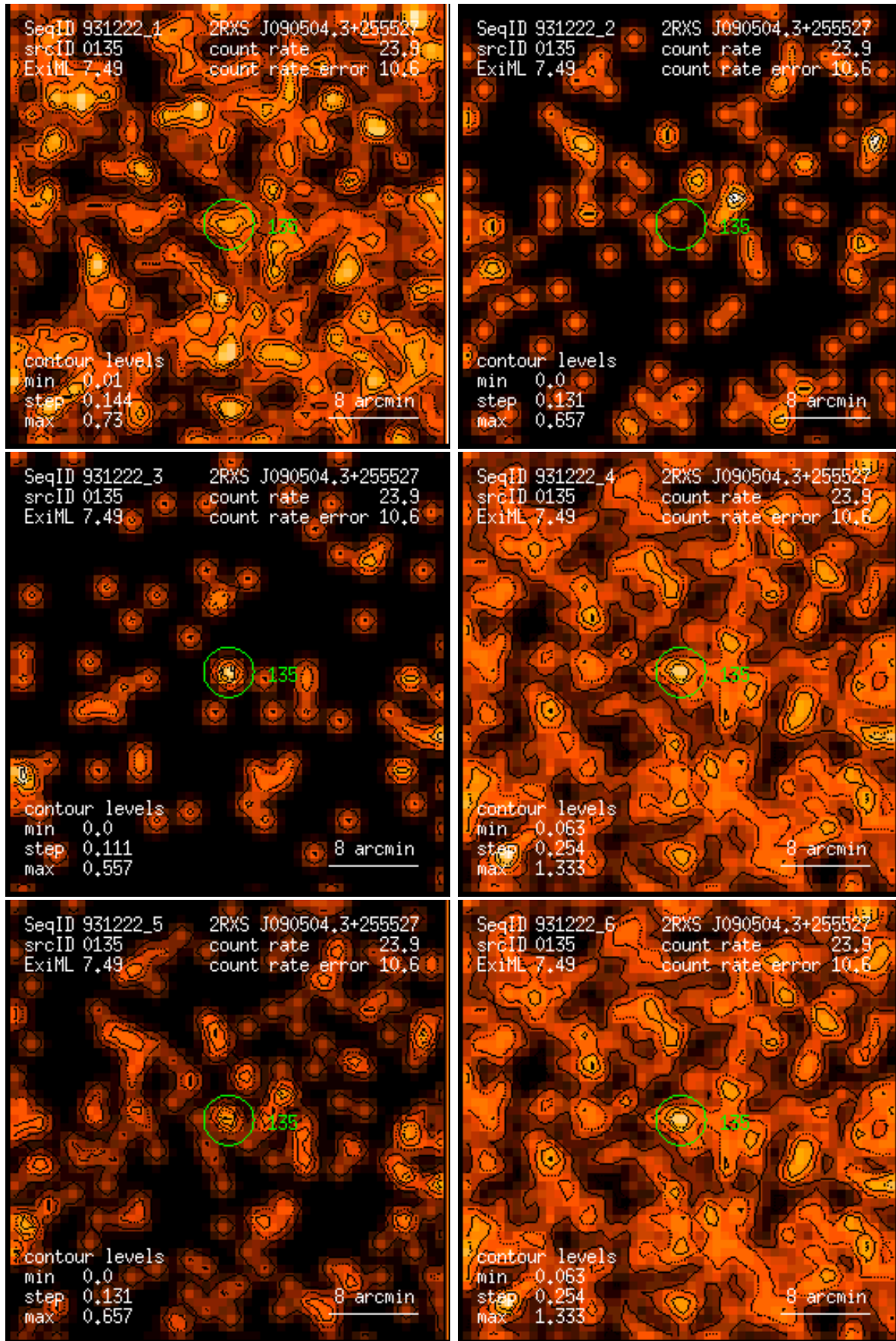
Figure 135: RASS 931222: detection 0135: band rate images, Gaussian filter: (1) PSPC channels 11 – 41, (2) 52 – 90, (3) 91 – 201, (4) 11 – 235, (5) 52 – 201, (6) 11 – 201. Broad band rates in counts/ks. Band rate contour levels in counts/ks/arcmin 2 .
