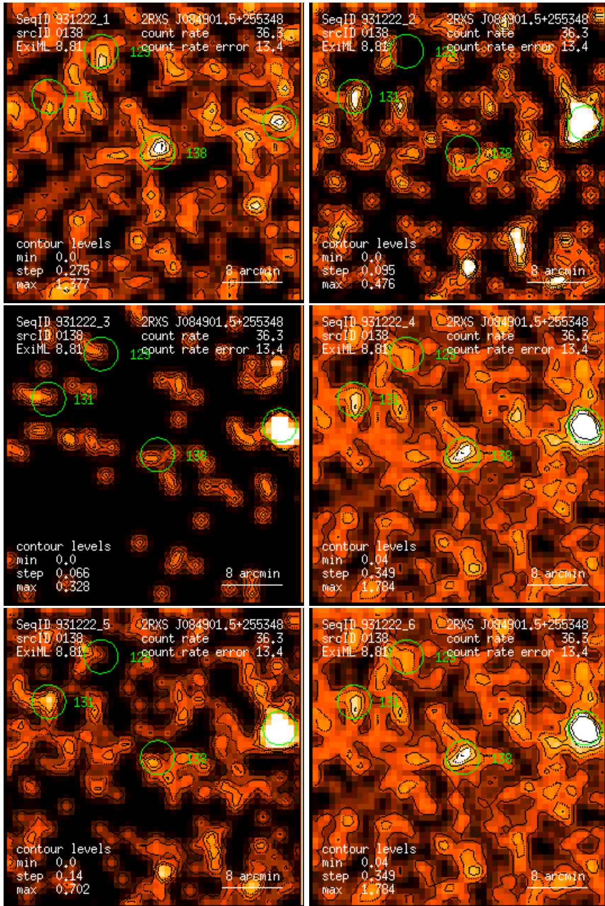
Figure 138: RASS 931222: detection 0138: band rate images, Gaussian filter: (1) PSPC channels 11 – 41, (2) 52 – 90, (3) 91 – 201, (4) 11 – 235, (5) 52 – 201, (6) 11 – 201. Broad band rates in counts/ks. Band rate contour levels in counts/ks/arcmin 2 .
