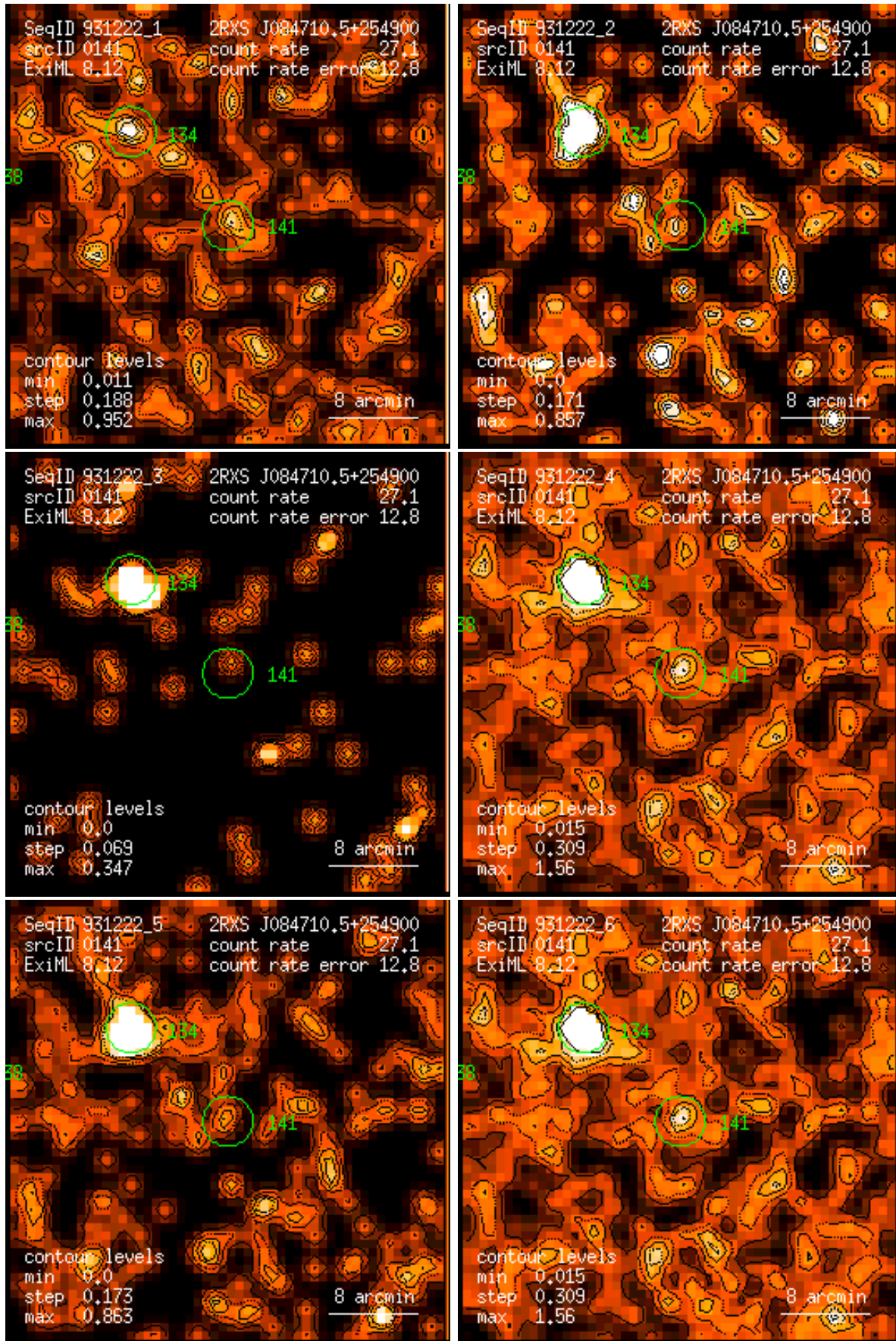
Figure 141: RASS 931222: detection 0141: band rate images, Gaussian filter: (1) PSPC channels 11 – 41, (2) 52 – 90, (3) 91 – 201, (4) 11 – 235, (5) 52 – 201, (6) 11 – 201. Broad band rates in counts/ks. Band rate contour levels in counts/ks/arcmin 2 .
