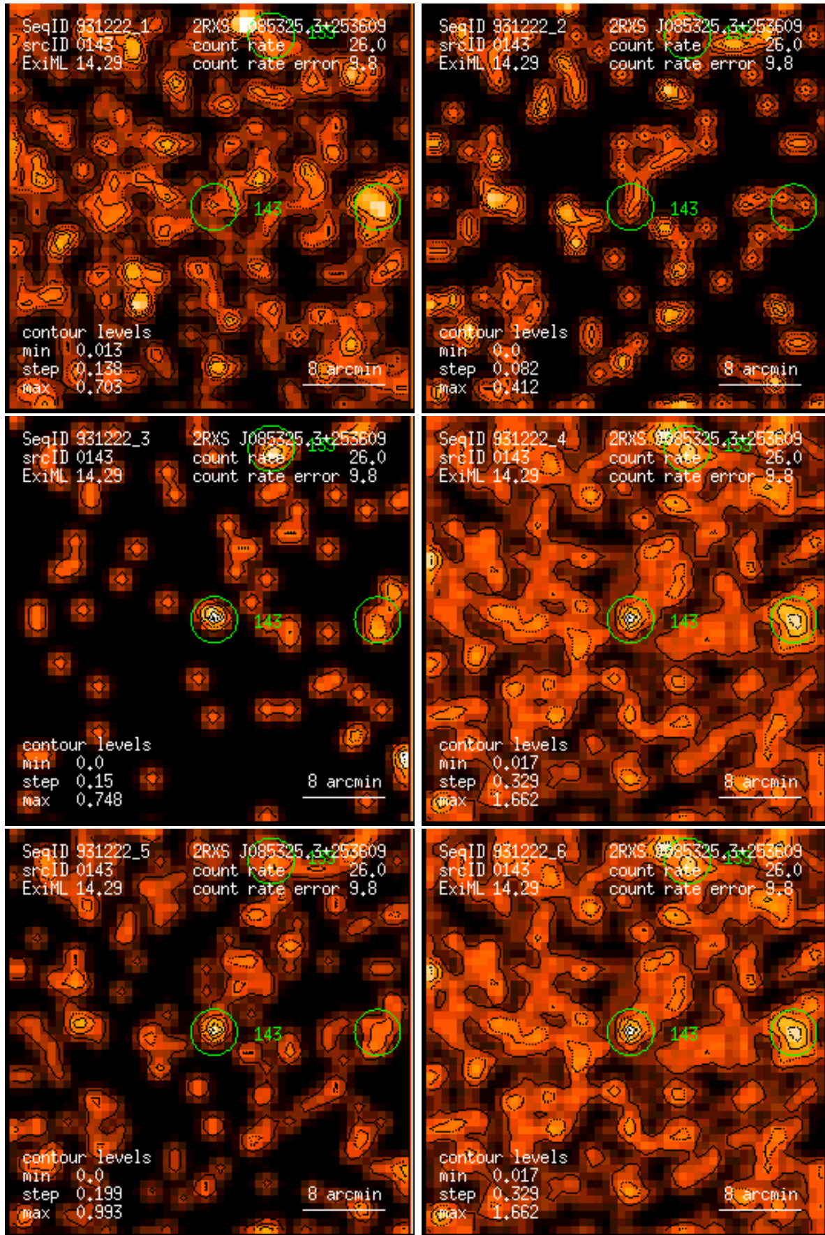
Figure 143: RASS 931222: detection 0143: band rate images, Gaussian filter: (1) PSPC channels 11 – 41, (2) 52 – 90, (3) 91 – 201, (4) 11 – 235, (5) 52 – 201, (6) 11 – 201. Broad band rates in counts/ks. Band rate contour levels in counts/ks/arcmin 2 .
