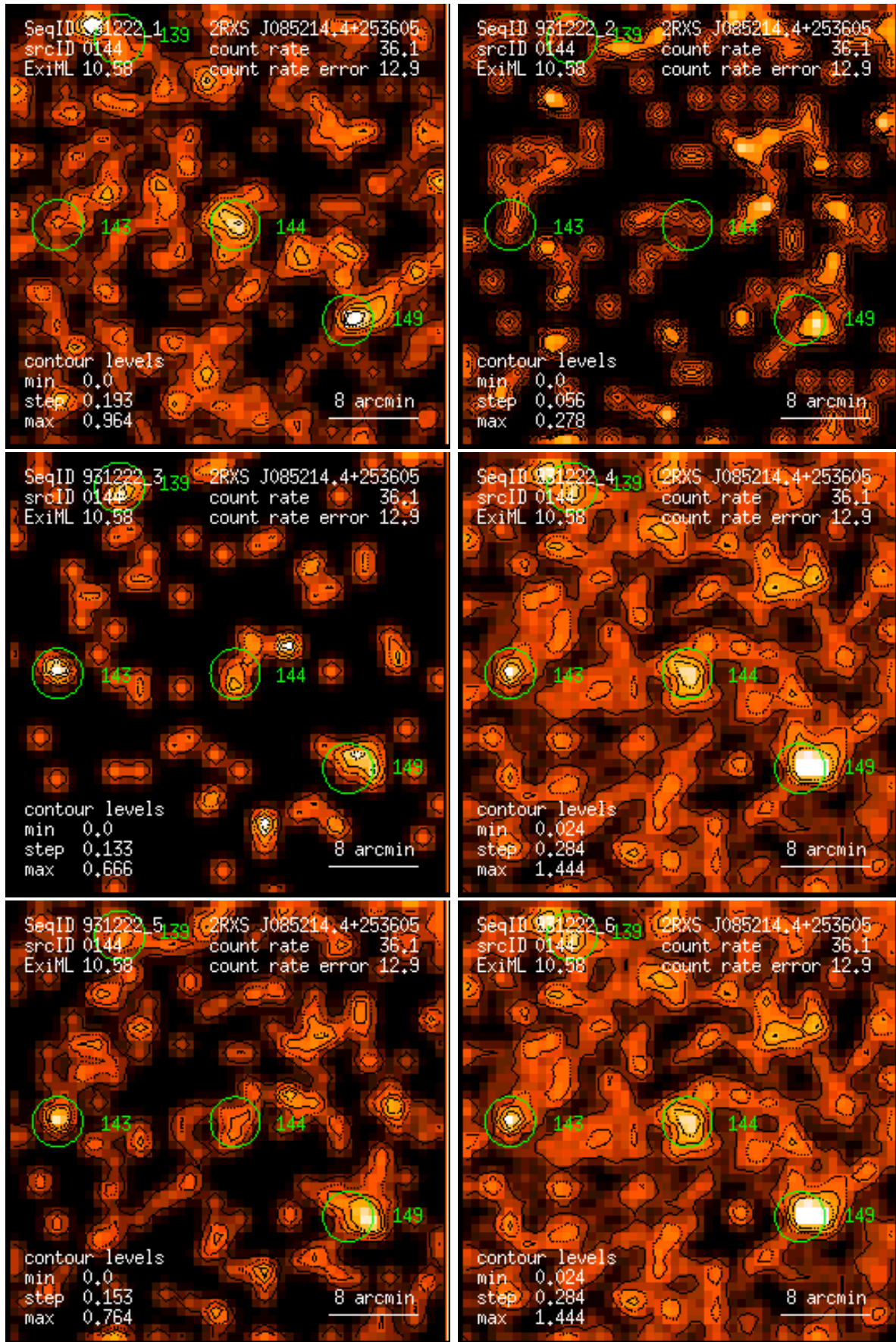
Figure 144: RASS 931222: detection 0144: band rate images, Gaussian filter: (1) PSPC channels 11 – 41, (2) 52 – 90, (3) 91 – 201, (4) 11 – 235, (5) 52 – 201, (6) 11 – 201. Broad band rates in counts/ks. Band rate contour levels in counts/ks/arcmin 2 .
