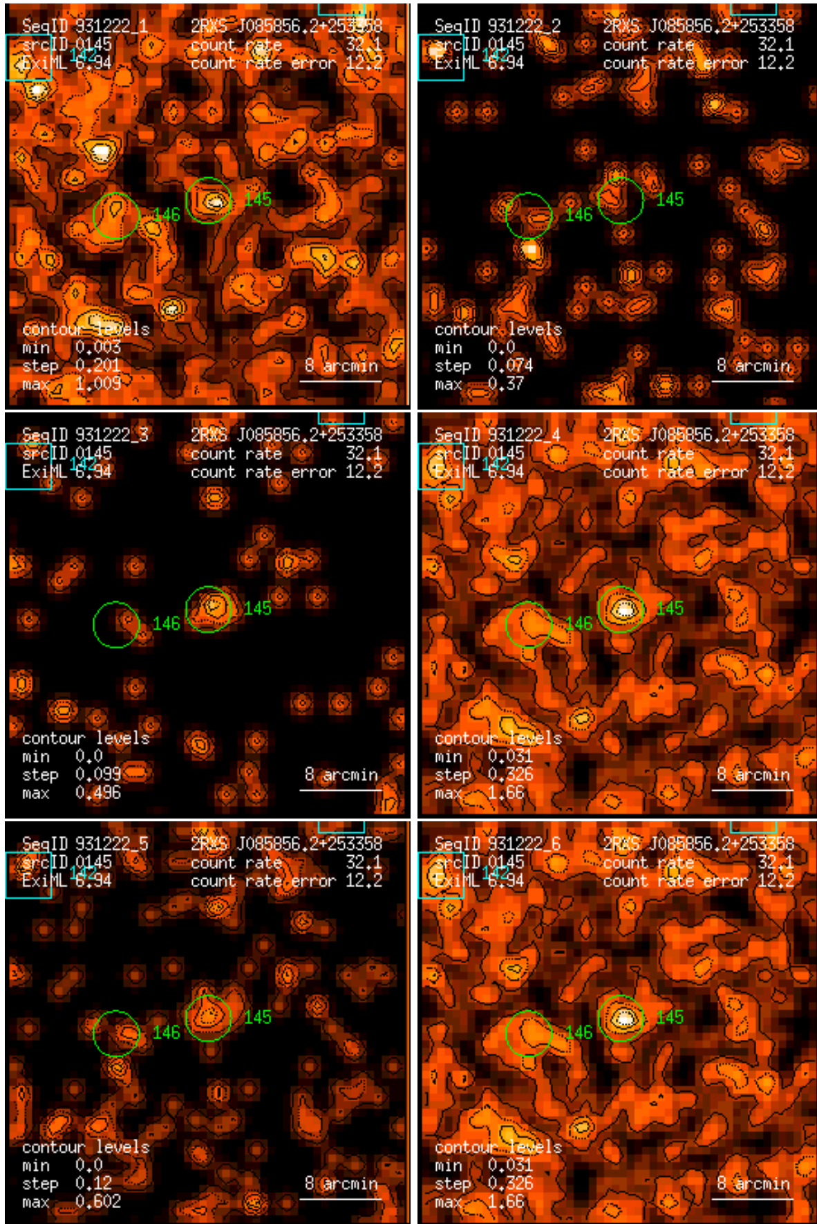
Figure 145: RASS 931222: detection 0145: band rate images, Gaussian filter: (1) PSPC channels 11 – 41, (2) 52 – 90, (3) 91 – 201, (4) 11 – 235, (5) 52 – 201, (6) 11 – 201. Broad band rates in counts/ks. Band rate contour levels in counts/ks/arcmin 2 .
