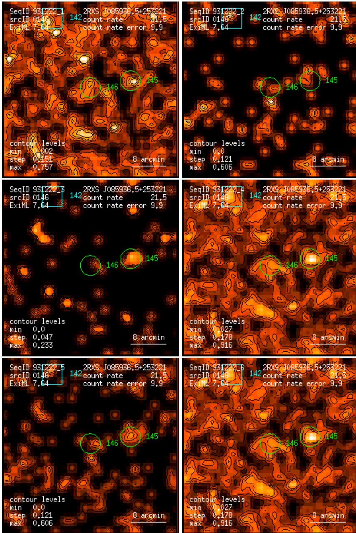
Figure 146: RASS 931222: detection 0146: band rate images, Gaussian filter: (1) PSPC channels 11 – 41, (2) 52 – 90, (3) 91 – 201, (4) 11 – 235, (5) 52 – 201, (6) 11 – 201. Broad band rates in counts/ks. Band rate contour levels in counts/ks/arcmin 2 .
