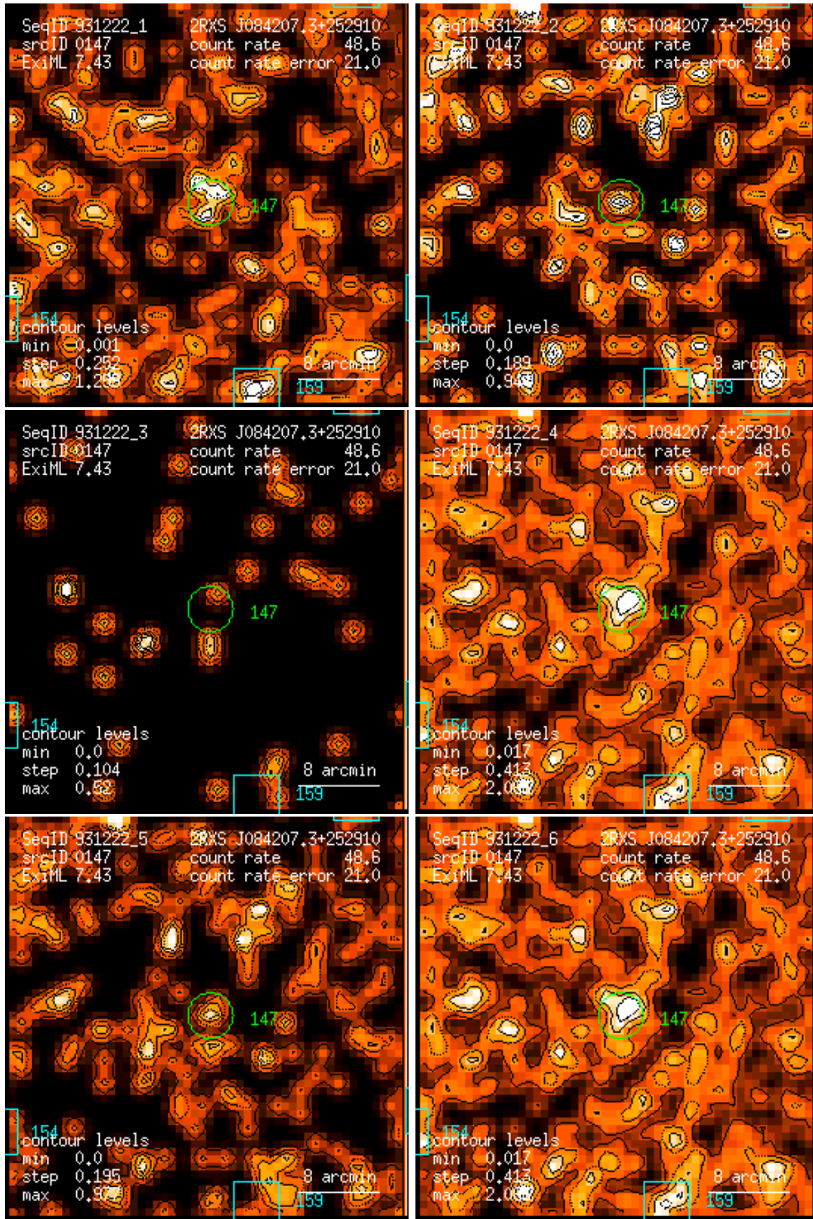
Figure 147: RASS 931222: detection 0147: band rate images, Gaussian filter: (1) PSPC channels 11 – 41, (2) 52 – 90, (3) 91 – 201, (4) 11 – 235, (5) 52 – 201, (6) 11 – 201. Broad band rates in counts/ks. Band rate contour levels in counts/ks/arcmin 2 .
