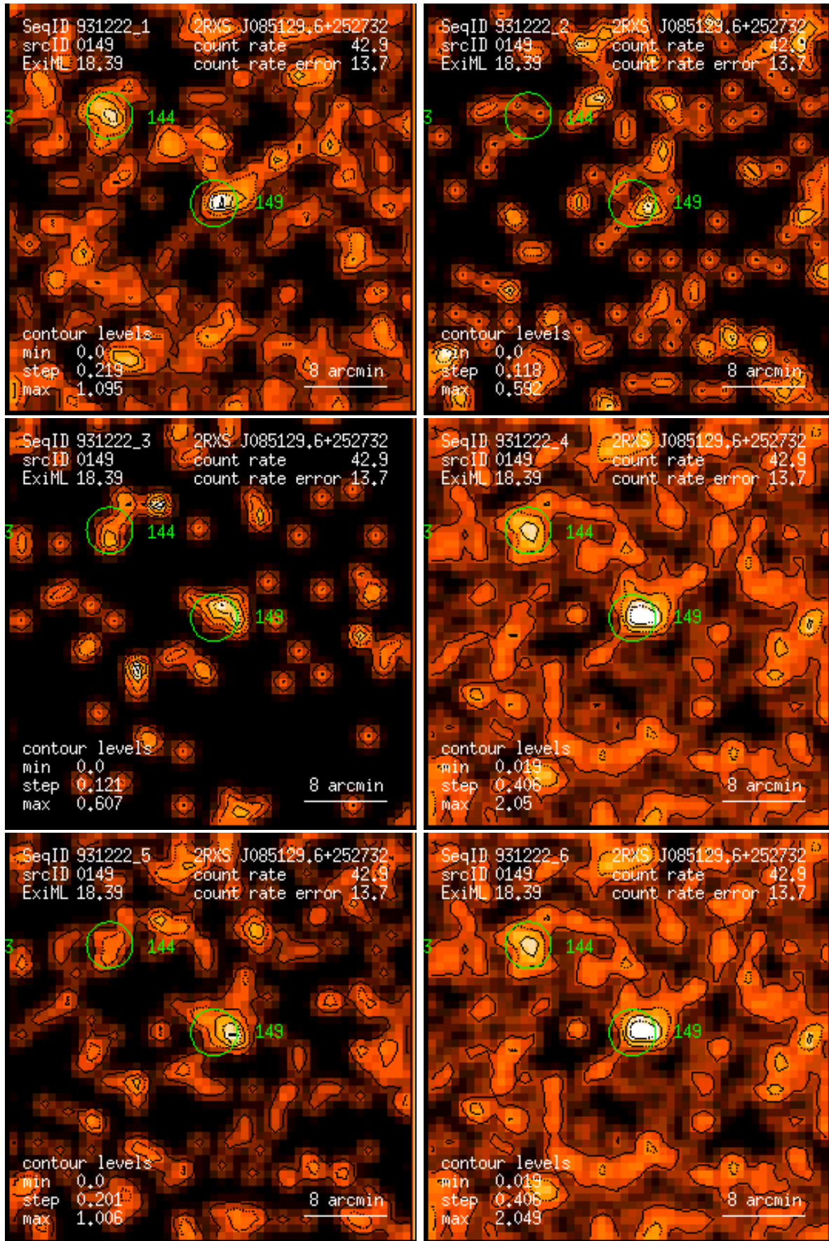
Figure 149: RASS 931222: detection 0149: band rate images, Gaussian filter: (1) PSPC channels 11 – 41, (2) 52 – 90, (3) 91 – 201, (4) 11 – 235, (5) 52 – 201, (6) 11 – 201. Broad band rates in counts/ks. Band rate contour levels in counts/ks/arcmin 2 .
