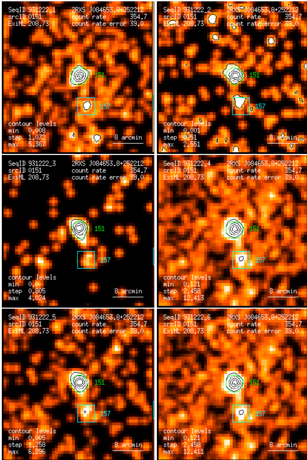
Figure 151: RASS 931222: detection 0151: band rate images, Gaussian filter: (1) PSPC channels 11 – 41, (2) 52 – 90, (3) 91 – 201, (4) 11 – 235, (5) 52 – 201, (6) 11 – 201. Broad band rates in counts/ks. Band rate contour levels in counts/ks/arcmin 2 .
