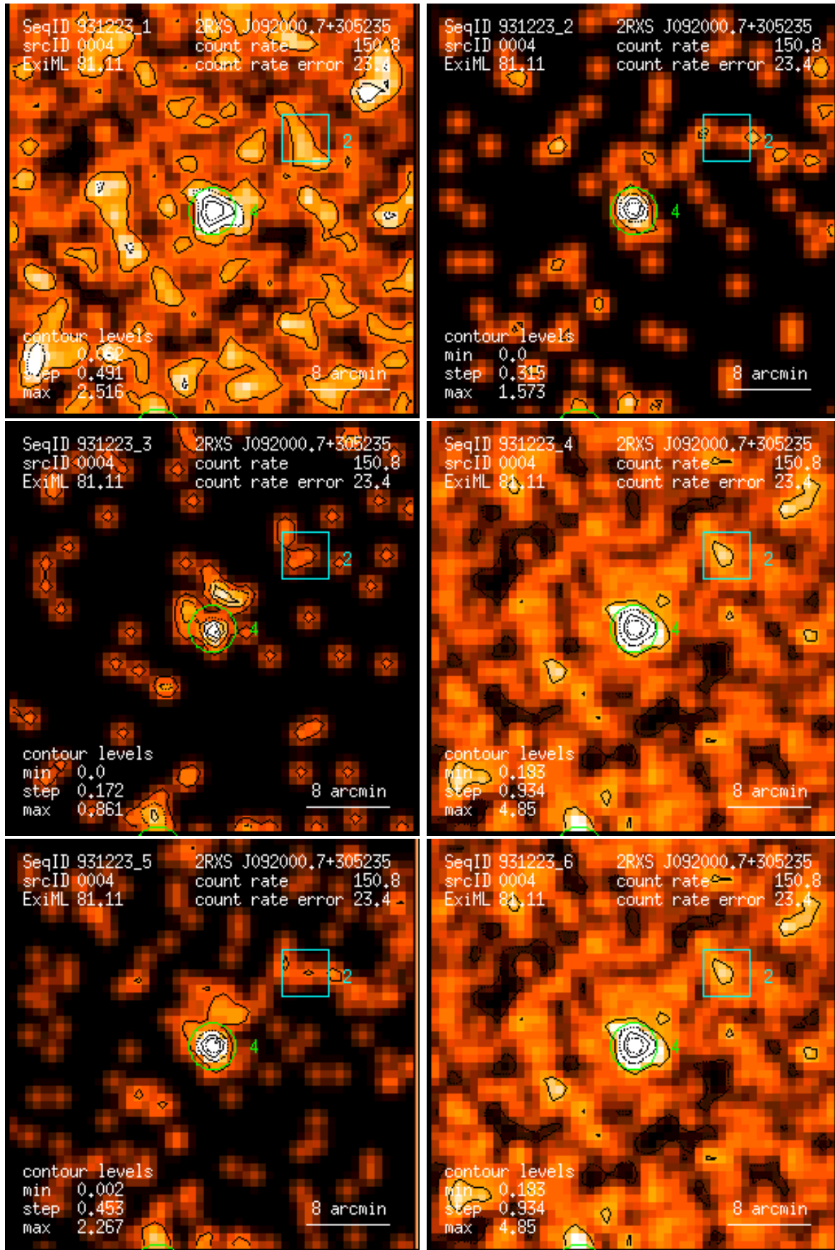
Figure 4: RASS 931223: detection 0004: band rate images, Gaussian filter: (1) PSPC channels 11 – 41, (2) 52 – 90, (3) 91 – 201, (4) 11 – 235, (5) 52 – 201, (6) 11 – 201. Broad band rates in counts/ks. Band rate contour levels in counts/ks/arcmin 2 .
