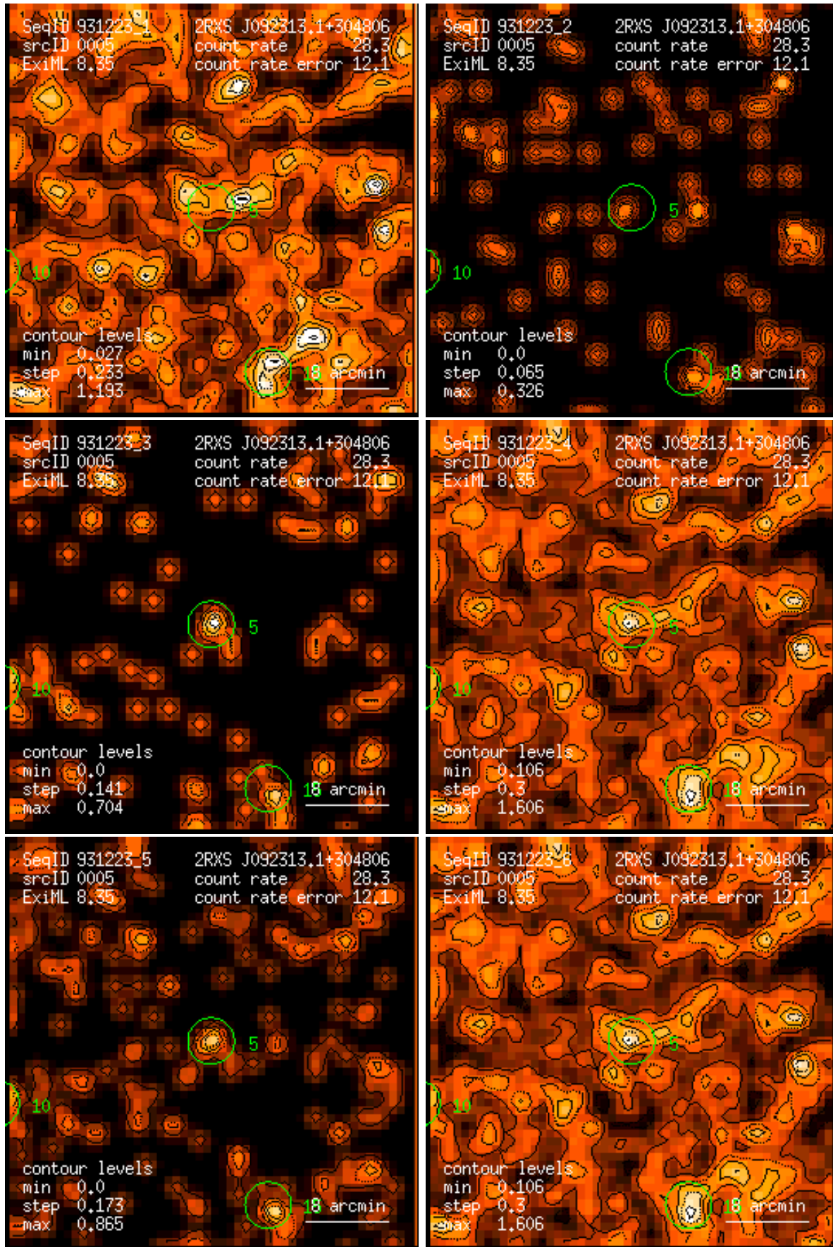
Figure 5: RASS 931223: detection 0005: band rate images, Gaussian filter: (1) PSPC channels 11 – 41, (2) 52 – 90, (3) 91 – 201, (4) 11 – 235, (5) 52 – 201, (6) 11 – 201. Broad band rates in counts/ks. Band rate contour levels in counts/ks/arcmin 2 .
