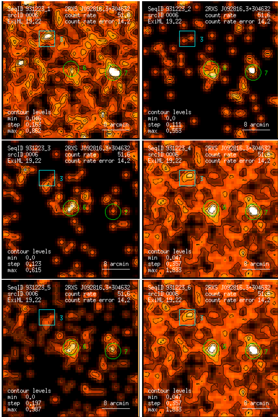
Figure 6: RASS 931223: detection 0006: band rate images, Gaussian filter: (1) PSPC channels 11 – 41, (2) 52 – 90, (3) 91 – 201, (4) 11 – 235, (5) 52 – 201, (6) 11 – 201. Broad band rates in counts/ks. Band rate contour levels in counts/ks/arcmin 2 .
