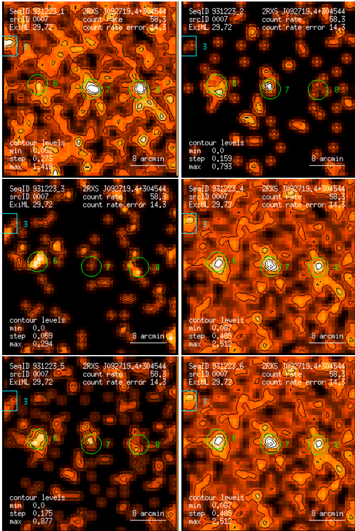
Figure 7: RASS 931223: detection 0007: band rate images, Gaussian filter: (1) PSPC channels 11 – 41, (2) 52 – 90, (3) 91 – 201, (4) 11 – 235, (5) 52 – 201, (6) 11 – 201. Broad band rates in counts/ks. Band rate contour levels in counts/ks/arcmin 2 .
