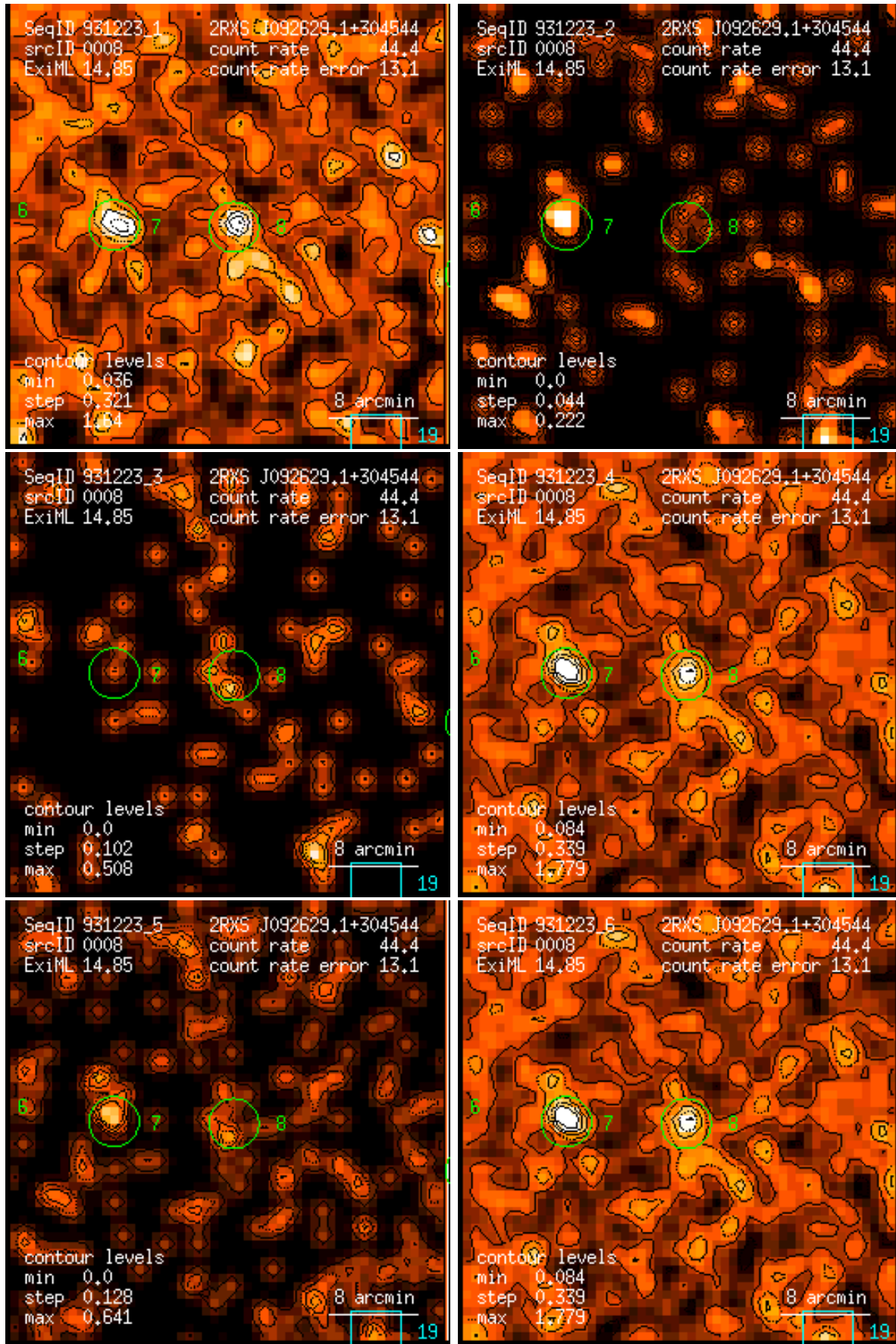
Figure 8: RASS 931223: detection 0008: band rate images, Gaussian filter: (1) PSPC channels 11 – 41, (2) 52 – 90, (3) 91 – 201, (4) 11 – 235, (5) 52 – 201, (6) 11 – 201. Broad band rates in counts/ks. Band rate contour levels in counts/ks/arcmin 2 .
