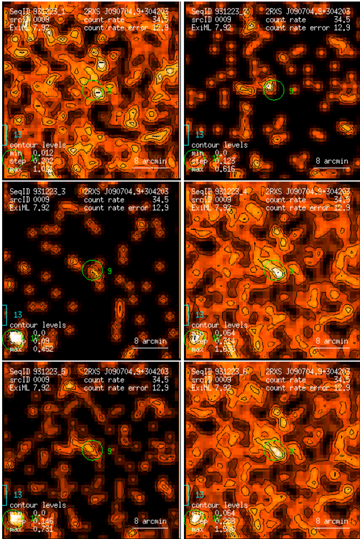
Figure 9: RASS 931223: detection 0009: band rate images, Gaussian filter: (1) PSPC channels 11 – 41, (2) 52 – 90, (3) 91 – 201, (4) 11 – 235, (5) 52 – 201, (6) 11 – 201. Broad band rates in counts/ks. Band rate contour levels in counts/ks/arcmin 2 .
