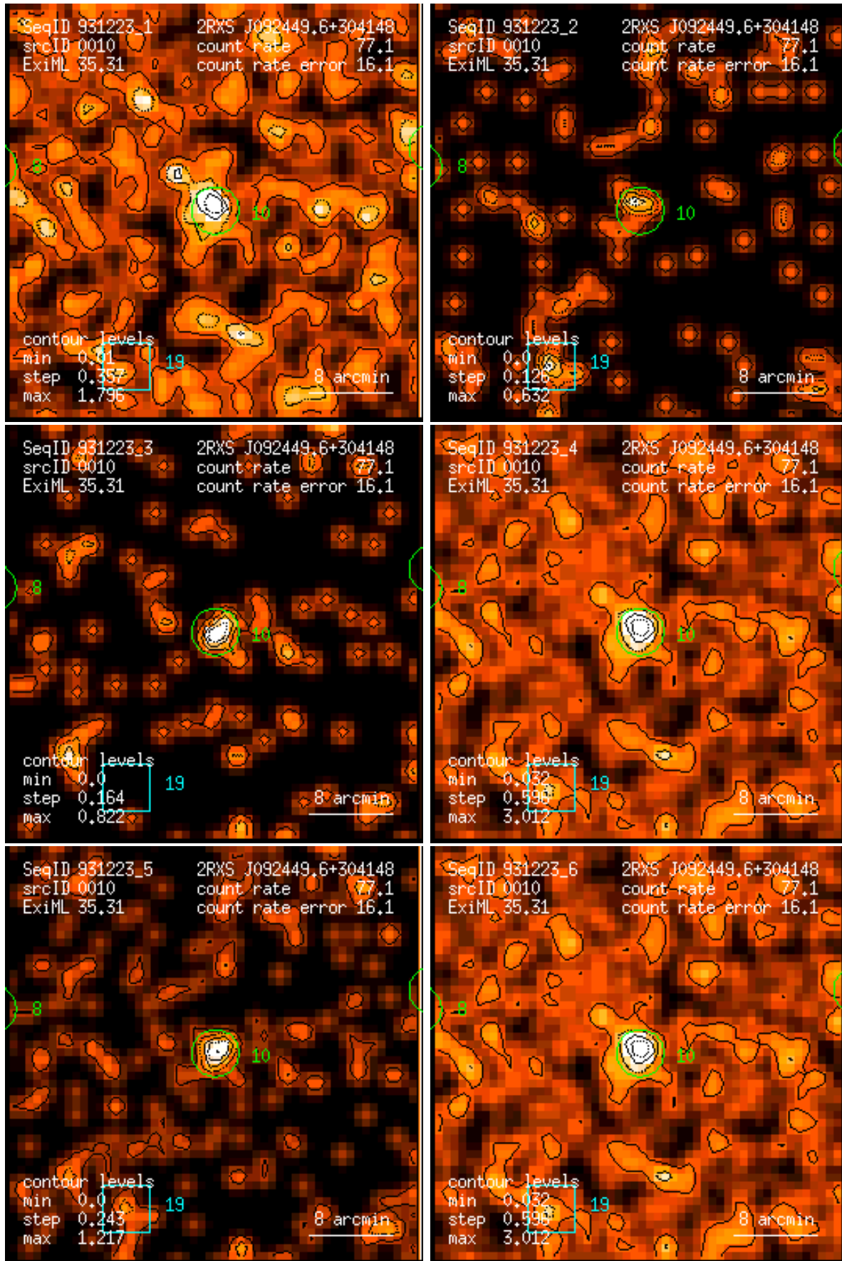
Figure 10: RASS 931223: detection 0010: band rate images, Gaussian filter: (1) PSPC channels 11 – 41, (2) 52 – 90, (3) 91 – 201, (4) 11 – 235, (5) 52 – 201, (6) 11 – 201. Broad band rates in counts/ks. Band rate contour levels in counts/ks/arcmin 2 .
